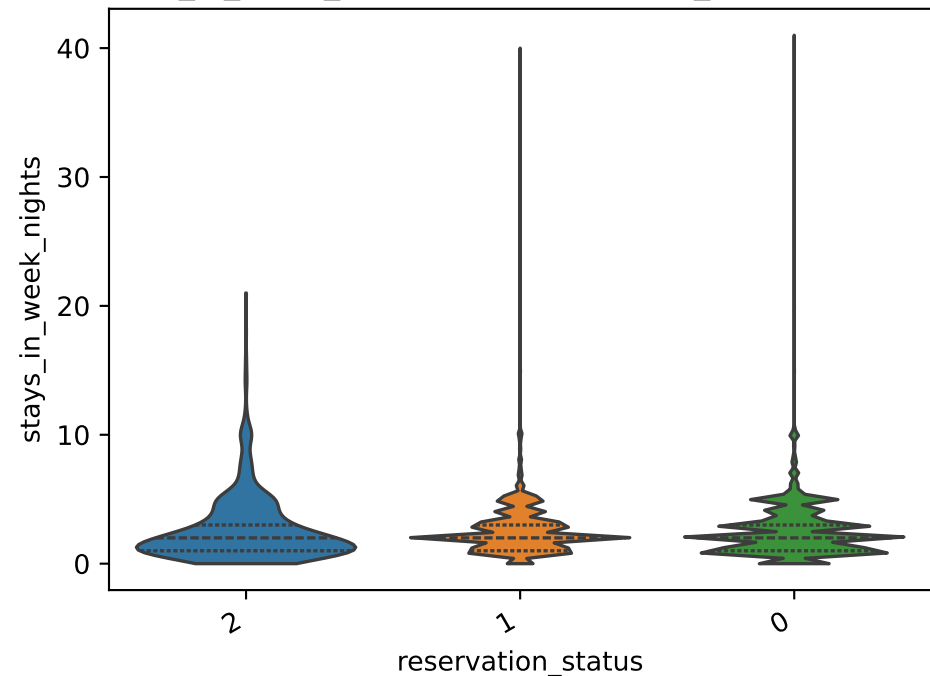
stays_in_week_nights par reservation_status (violins)
