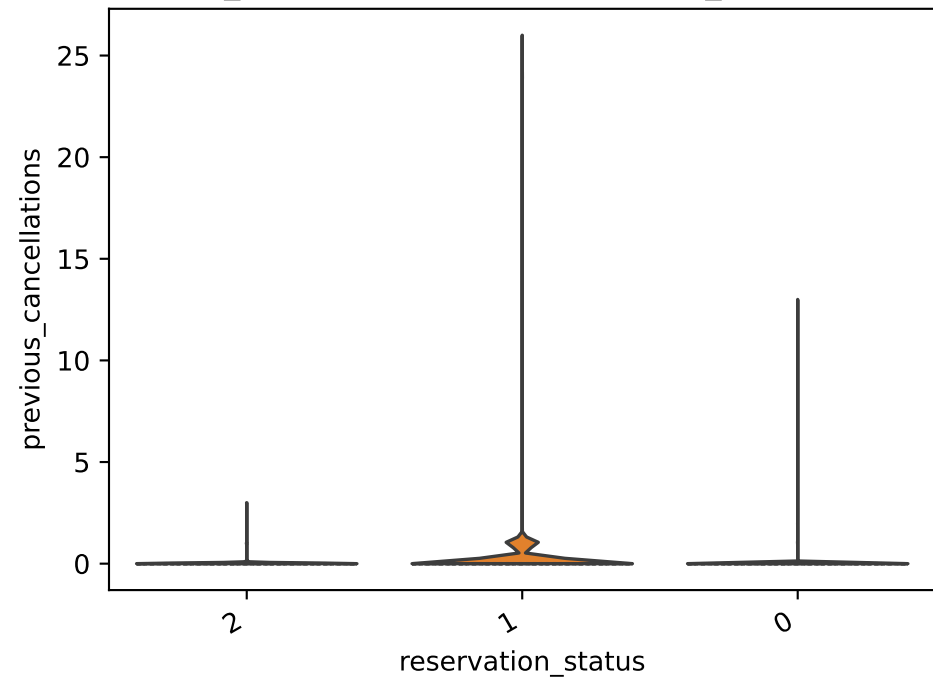
previous_cancellations par reservation_status (violins)
