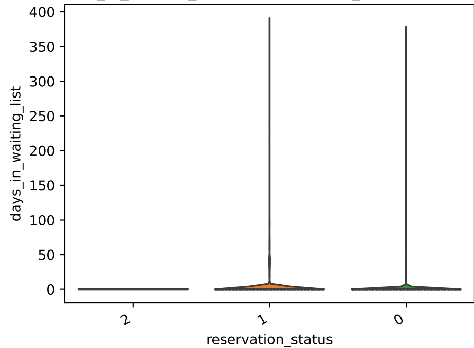
days_in_waiting_list par reservation_status (violins)
