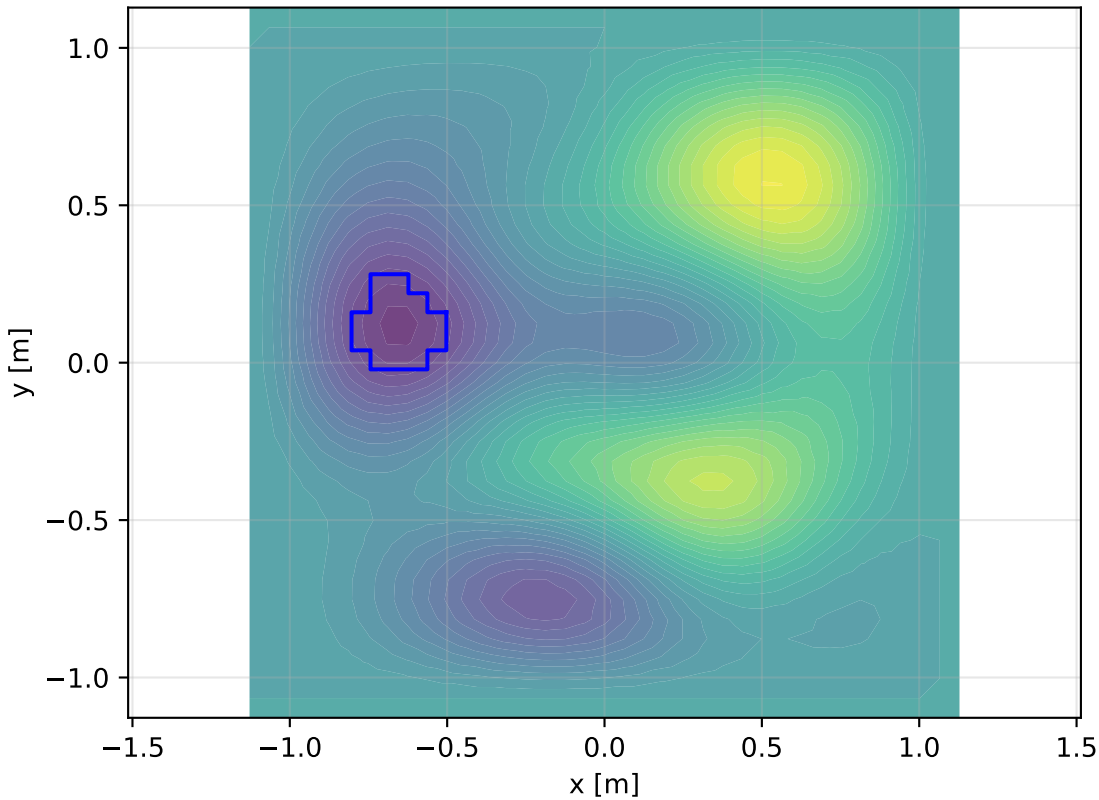
Face 2: xy-plane - Contour 0
