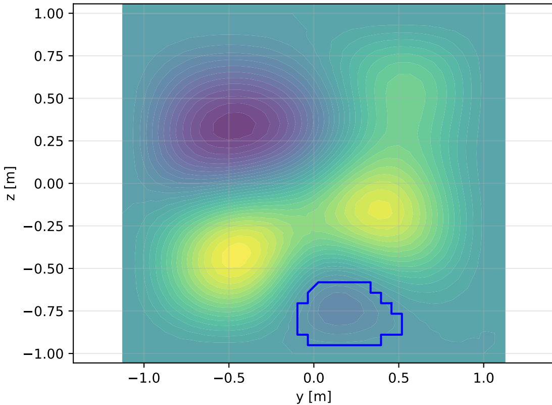
Face 6: yz-plane - Contour 6
