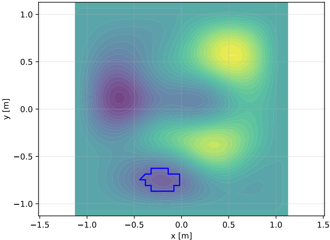
Face 2: xy-plane - Contour 4
