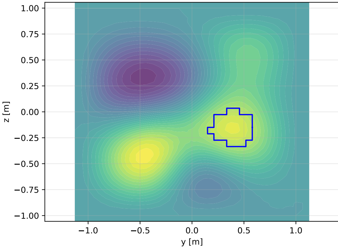
Face 6: yz-plane - Contour 12
