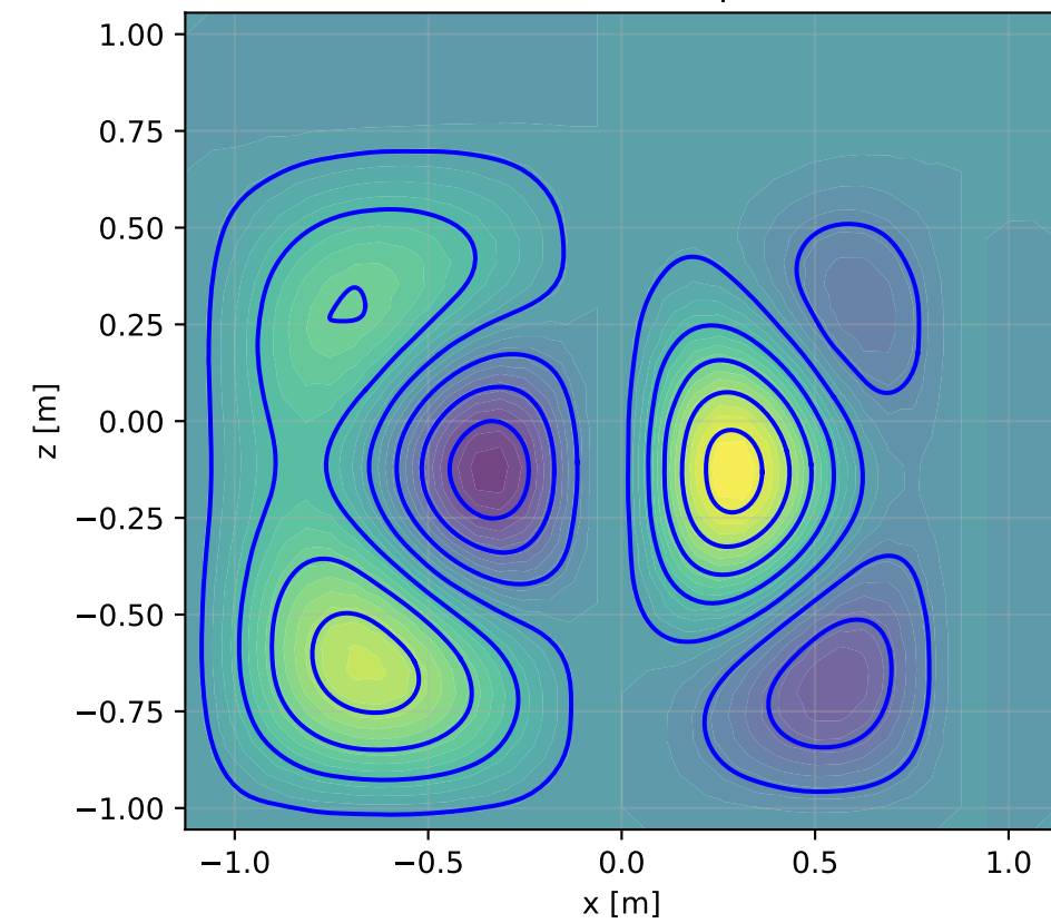
Face 4: Front (xz-plane)
