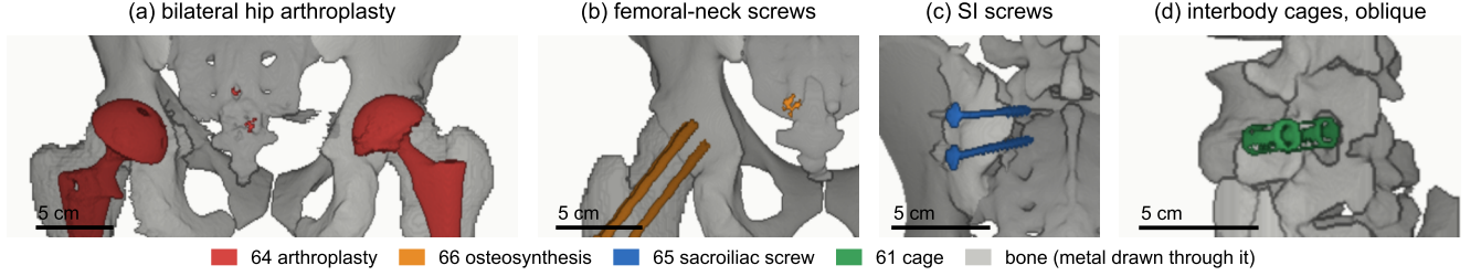
FIG. 3 Instrumentation in the release, one exemplar each, drawn through bone. (a) Hip arthroplasty, 64, n = 8 . (b) Femoral-neck screws, 66, n = 1 . (c) Sacroiliac screws, 65, n = 1 . (d) Interbody cages, 61, n = 1 . Bar, 5 cm.
