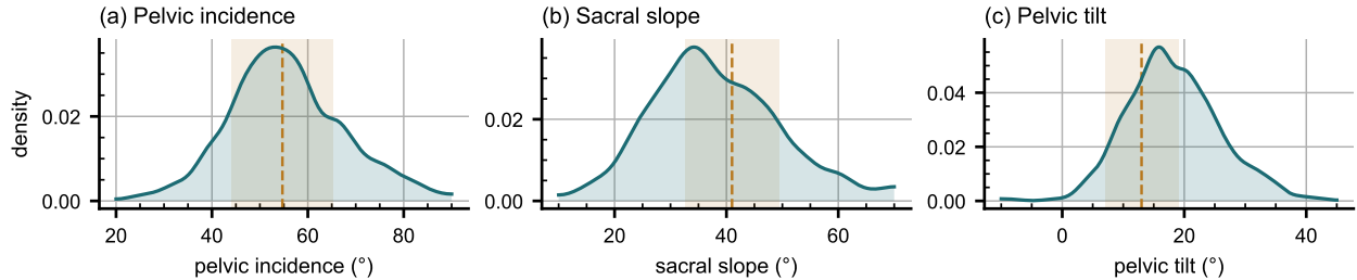
FIG. 5 Spinopelvic measures against standing reference bands (mean \pm SD) 31 .
