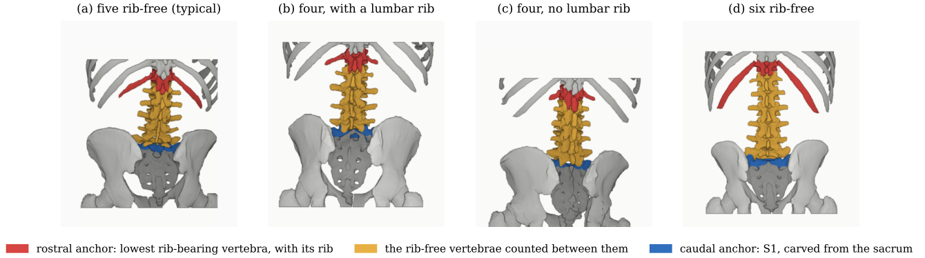
FIG. 2 The two anchors and the interval between them, from the released labels, posterior view. Rostral anchor: the lowest rib-bearing vertebra and the rib that makes it one. Caudal anchor: S1. Both are found from the labels rather than assumed, and panels are colored by role rather than identifier, since coloring T12 would assert the count the figure derives. Panels (b) and (c) reach the same interval of four from opposite ends and are indistinguishable by it. All panels are at one millimeter scale, aligned at the sacral base.
