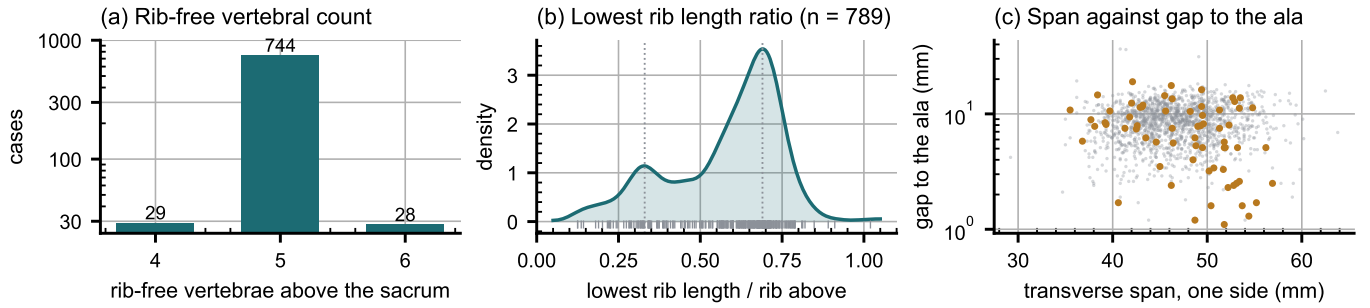
FIG. 4 Count-free measures. (a) Vertebrae between the lowest rib and the sacrum. (b) Lowest rib length over the rib above. (c) Lowest lumbar transverse span against its gap to the ala; transitional labels marked.
