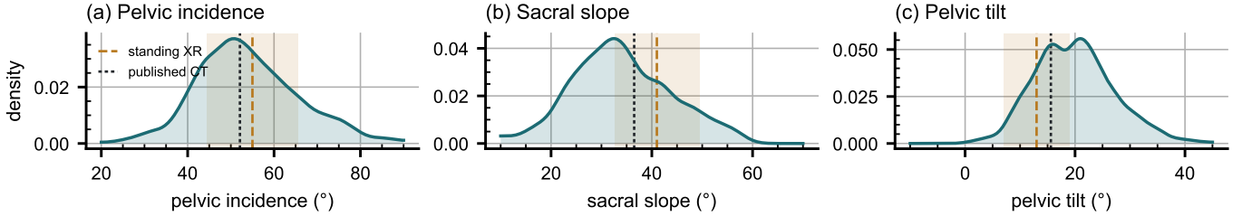
FIG. 5 Spinopelvic measures against standing reference bands (mean \pm SD) 37 .
