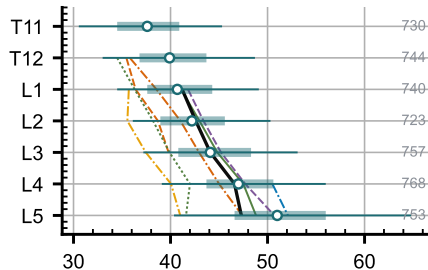
(a) Endplate width
