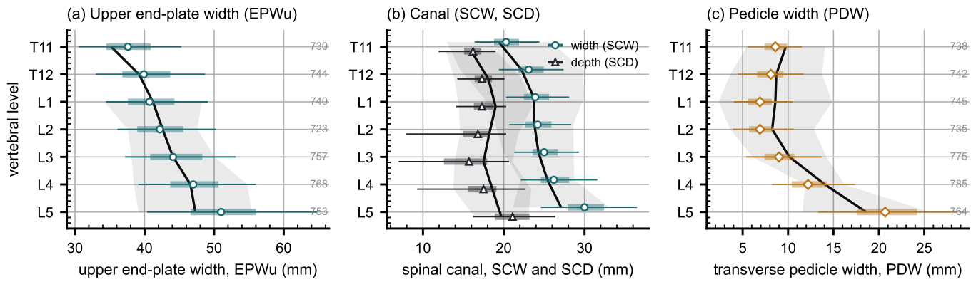
FIG. 6 Morphometry by level, T11–L5: median, interquartile range, 5th–95th percentile, n at right. (a) End-plate width EPWu. (b) Canal width SCW and depth SCD. (c) Pedicle width PDW, both sides averaged. Black lines are Panjabi's cadaveric means 24,25 ; grey bands his population interval, mean \pm 1.96 SD, SD recovered from the reported SEM ( n = 12 ). T11–T12 EPWu is digitised from his Figure 4A.
