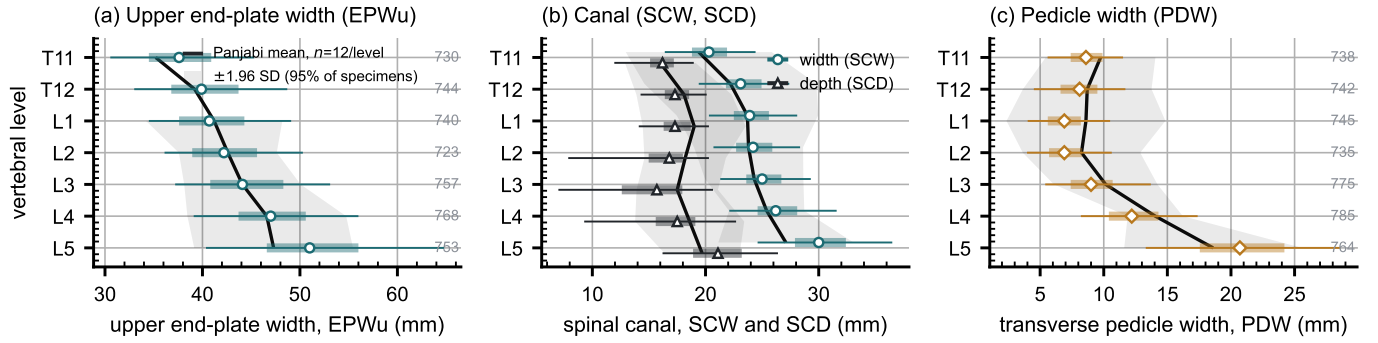
FIG. 6 Morphometry by level, T11–L5: median, interquartile range, 5th–95th percentile, n at right. (a) End-plate width EPWu. (b) Canal width SCW and depth SCD. (c) Pedicle width PDW, both sides averaged. Reference is Panjabi’s cadaveric series 25,26 , keyed in (a), its SD recovered from the reported SEM; T11–T12 EPWu is digitised from his Figure 4A.
