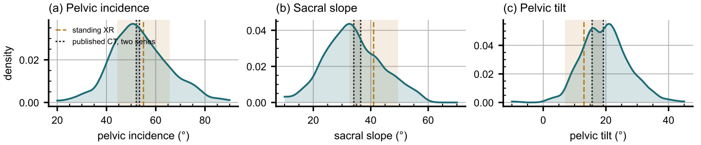
FIG. 5 Spinopelvic measures against standing reference bands (mean \pm SD) 37 .
