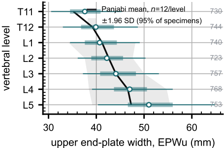
(a) Upper end-plate width (EPWu)
