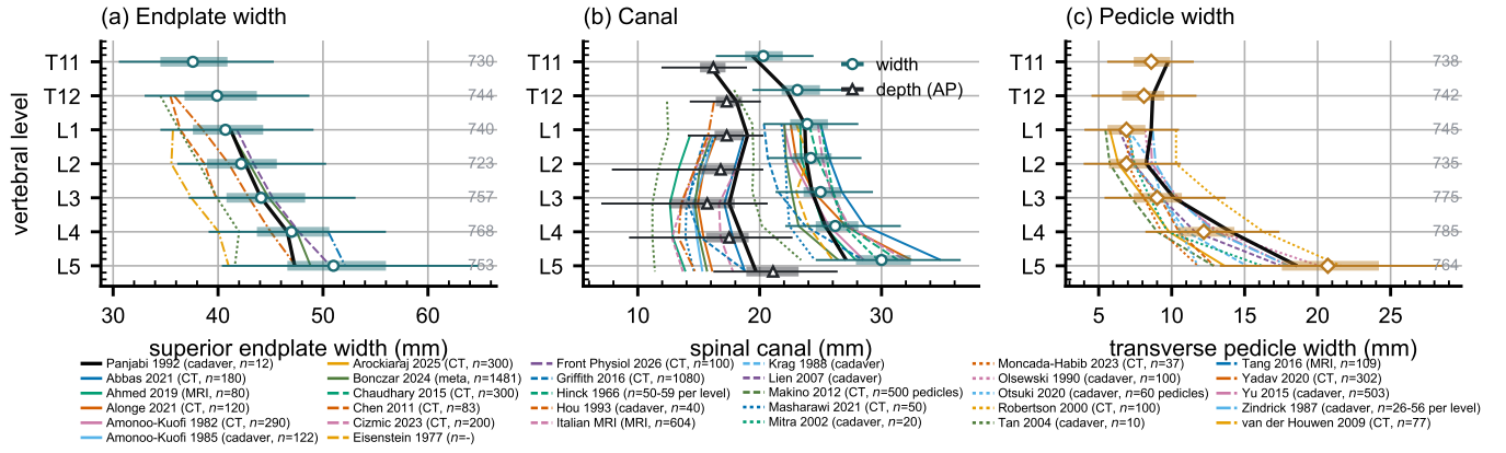
FIG. 6 Morphometry by level, T11–L5, as median, interquartile range and 5th–95th percentile, with n at right. (a) Endplate width. (b) Canal, width and depth. (c) Transverse pedicle width, the mean of the two sides. Lines are the published series for each measure, keyed below; Panjabi is drawn in black as the series the text cites.
