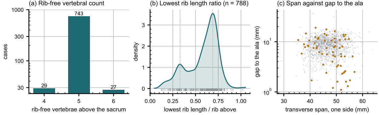
FIG. 4 Count-free measures. (a) Vertebrae between the lowest rib and the sacrum. (b) Lowest rib length over the rib above. (c) Lowest lumbar transverse span against its gap to the ala; transitional labels marked.
