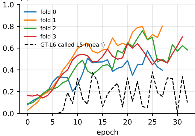
L6 Dice, six-lumbar validation cases (a) L6 is learned as its own class
