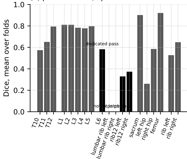
(b) per-class Dice, epochs 27-32 of 500
