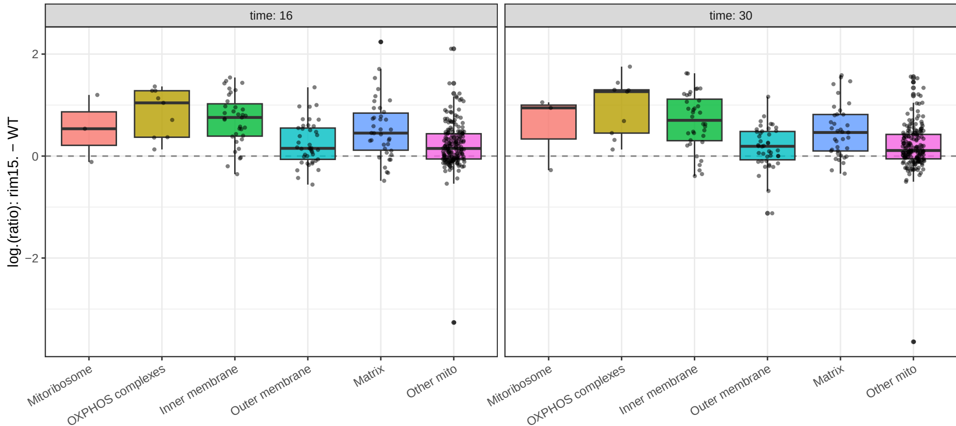
Genotype difference (rim15. – WT) in carbon starvation, by subcompartment
