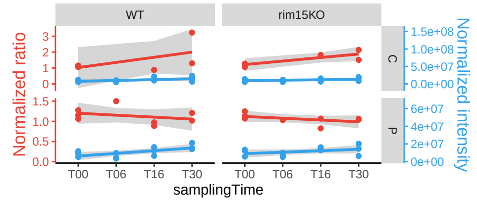
YDR476C
