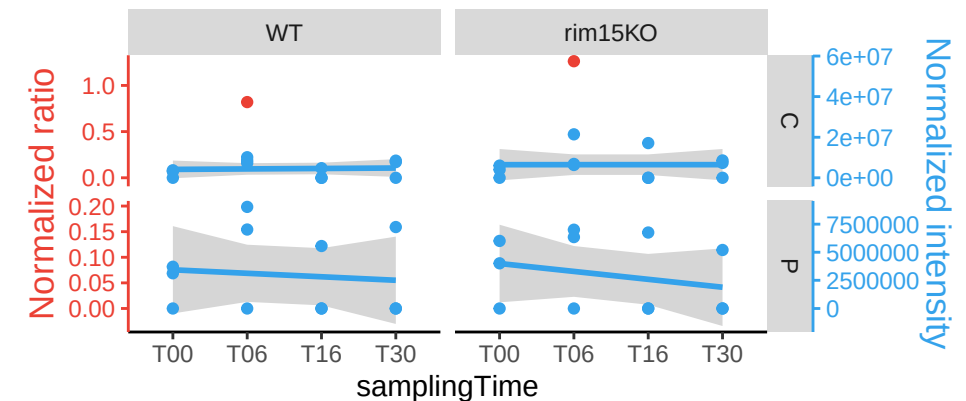
RPS25A;RPS25B
