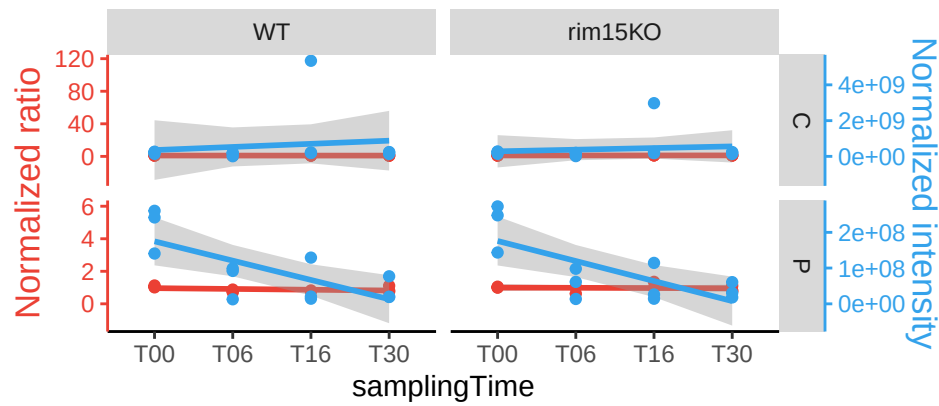
YET3
