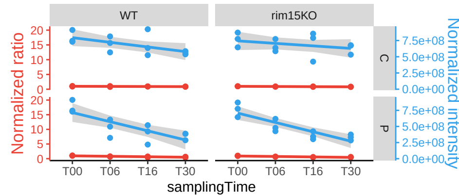
PMT1
