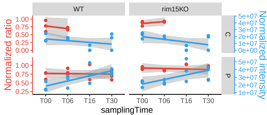
COA6
