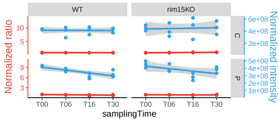
RPA12
