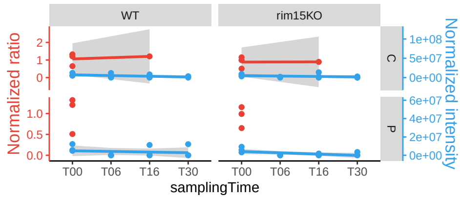
GAA1
