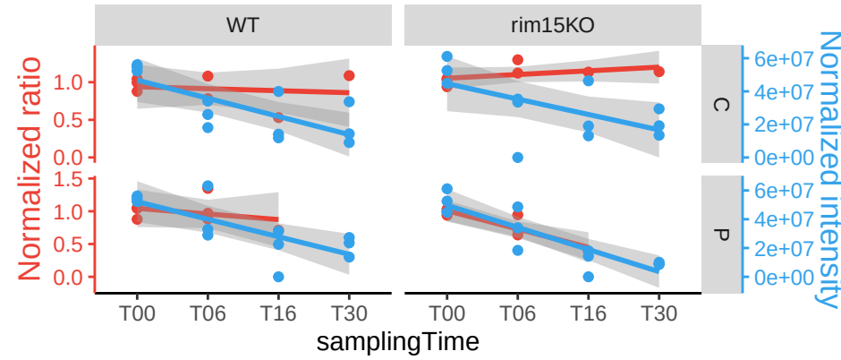
ATF2
