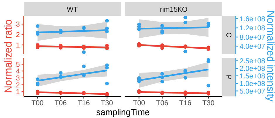
VMA7
