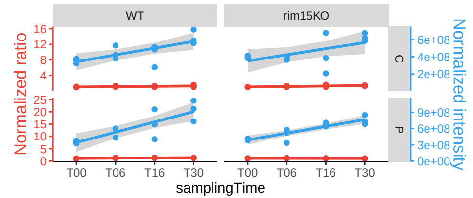
NAP1
