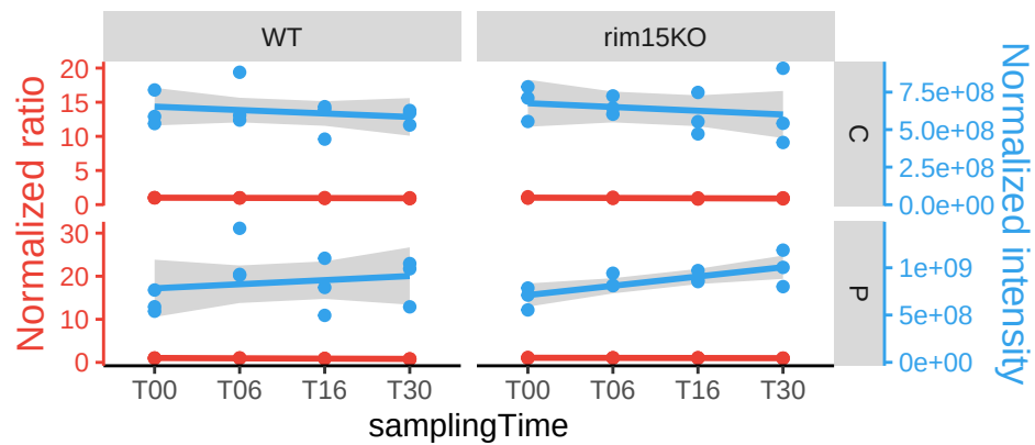
TRR1
