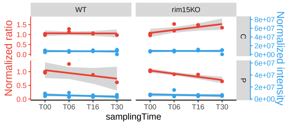
PMU1
