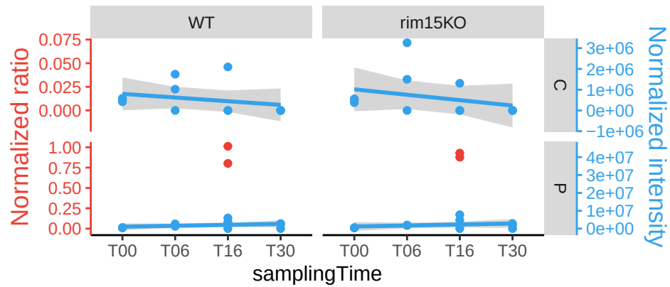
RMT2
