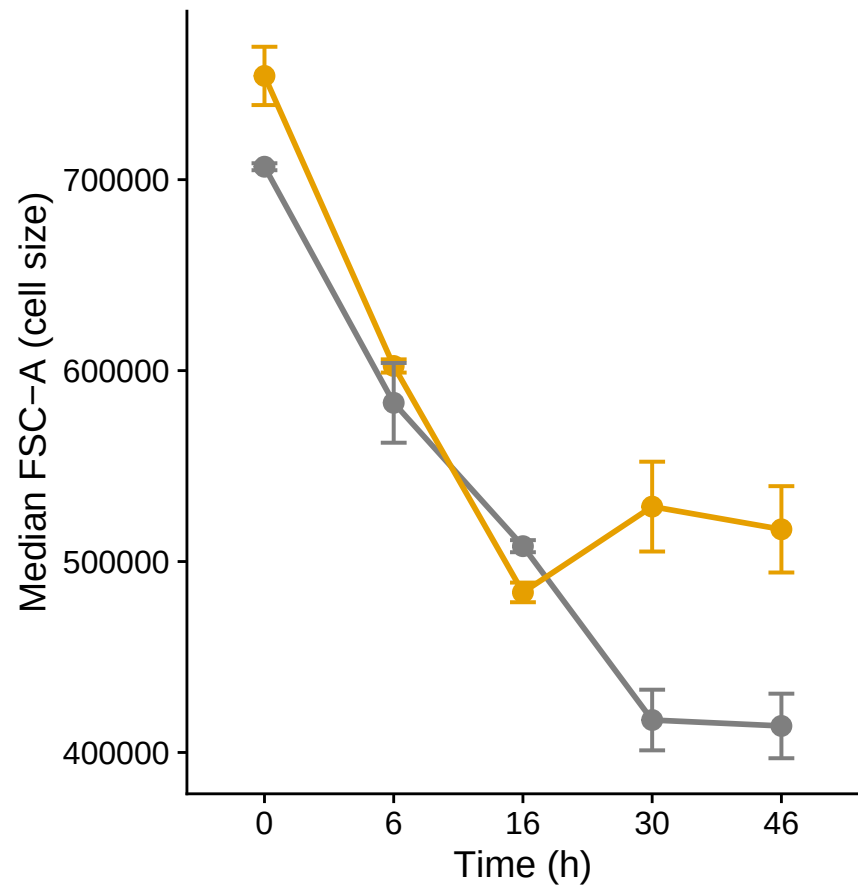
Carbon starvation
