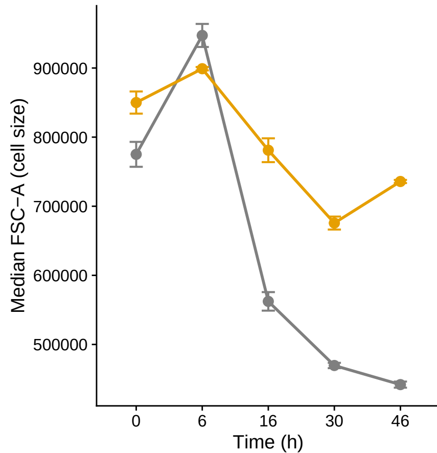
Nitrogen starvation
