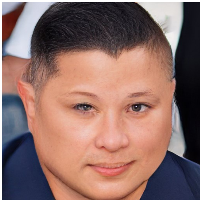
Face-SPARNet (approx. 32→512)
