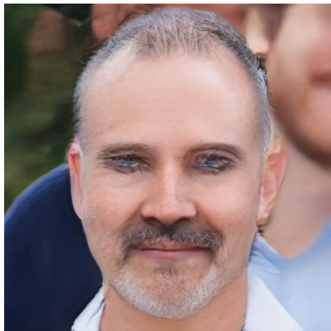
Face-SPARNet (approx. 32→512)
