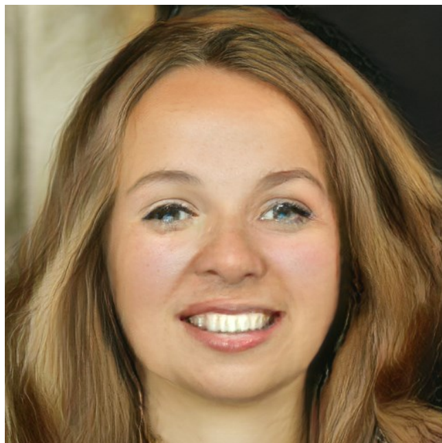
Face-SPARNet (approx. 32→512)
