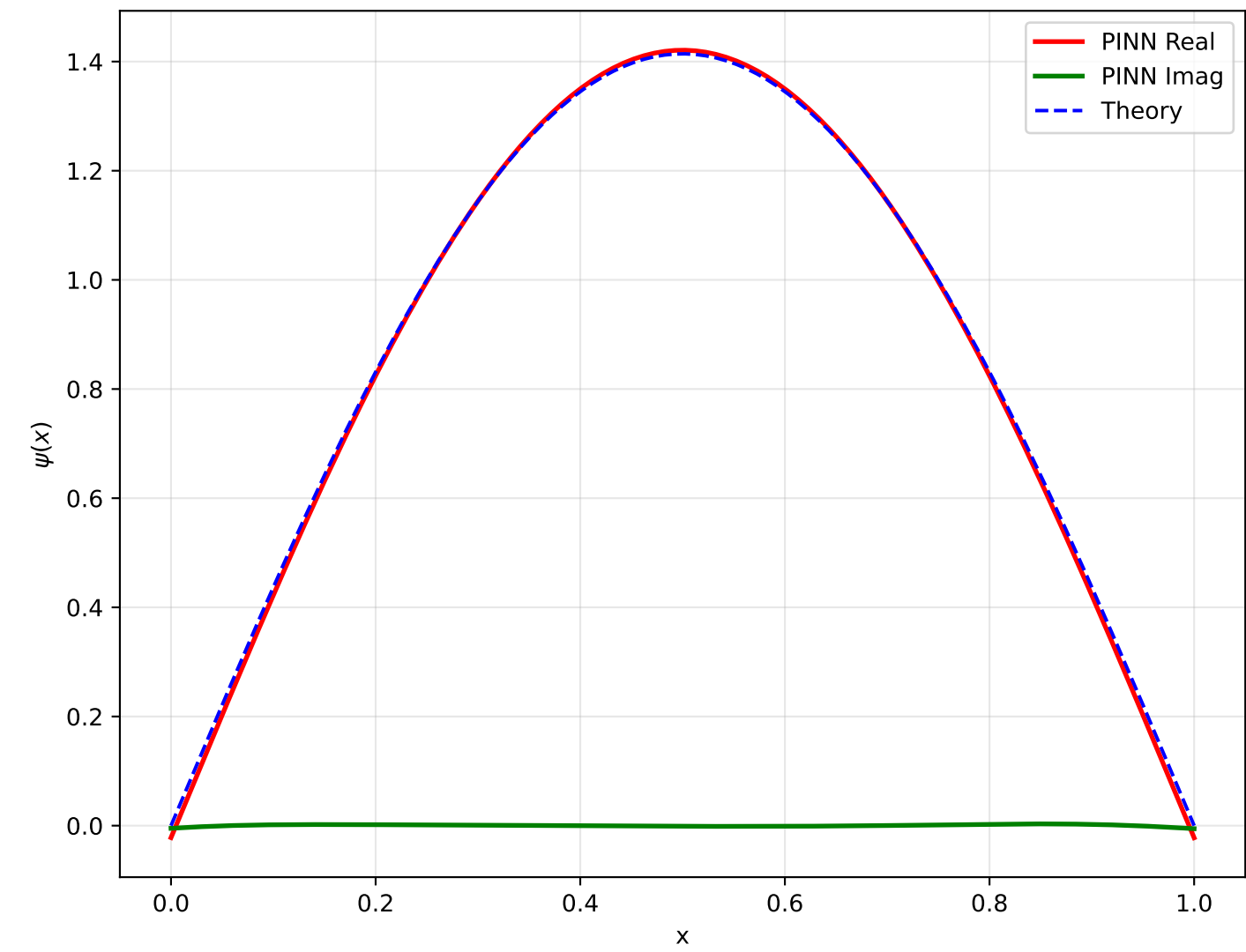
Wavefunction at t=0
