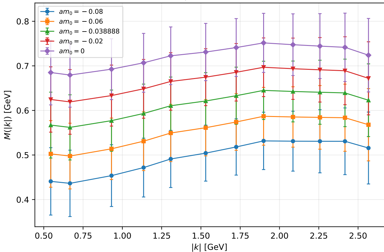
CG+IPG quark mass function
