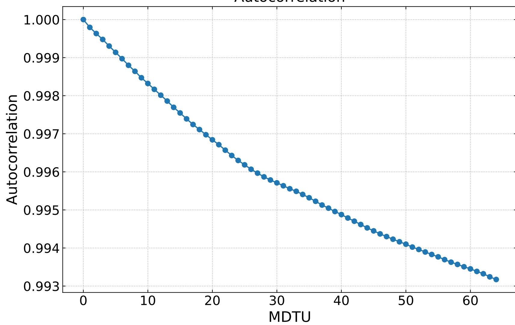
Autocorrelation
