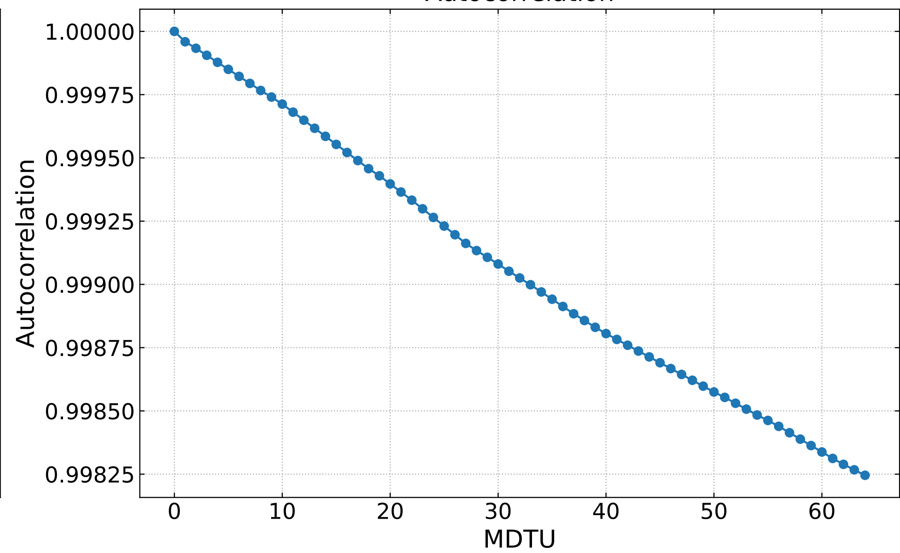
Autocorrelation
