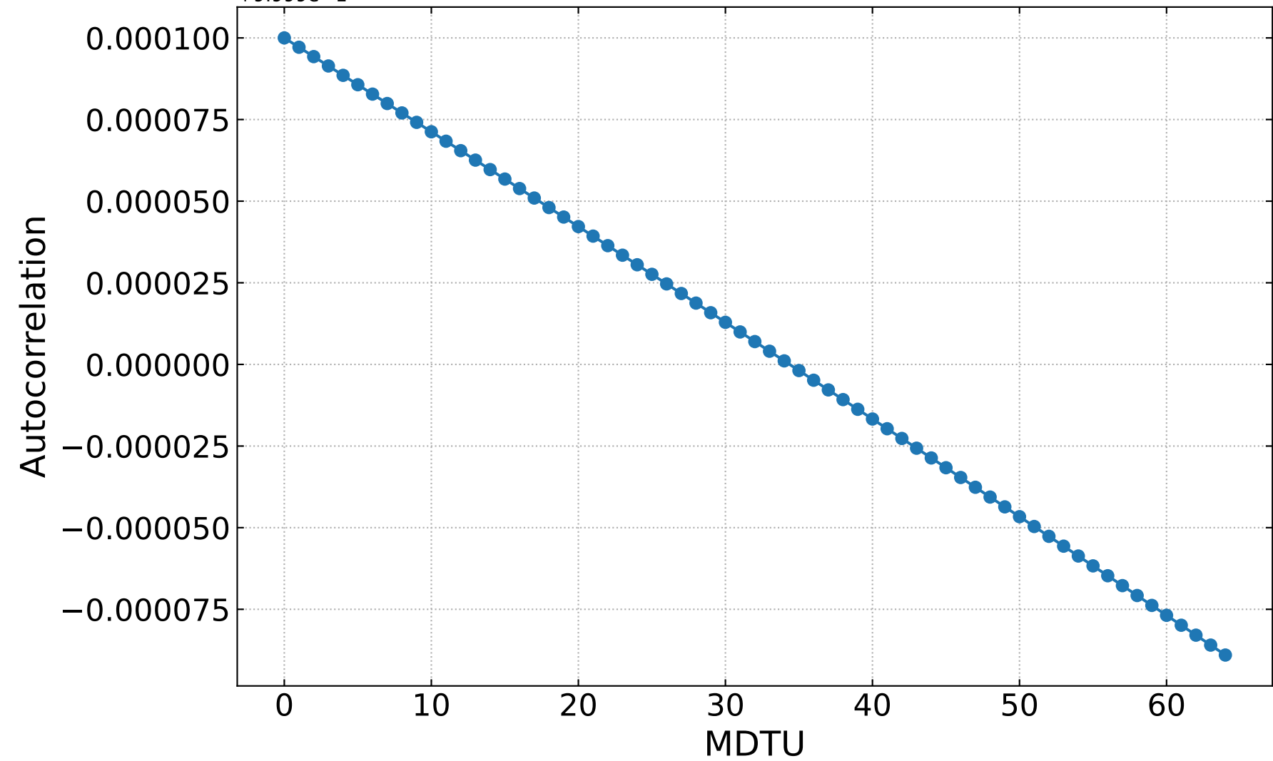
Autocorrelation
