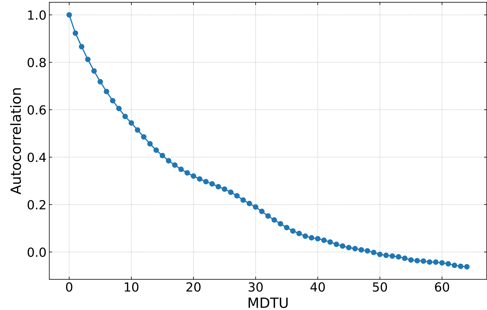
Autocorrelation
