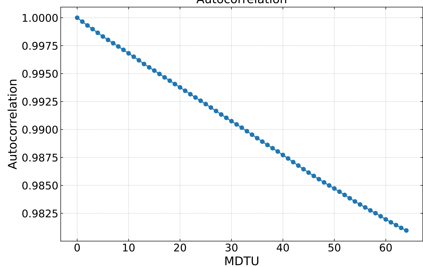
Autocorrelation
