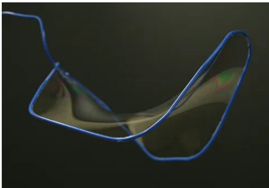
Figure 1: A soap film on a wire frame.
