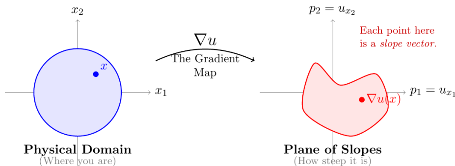
Figure 5: The Gradient Map. This map takes a location x in the physical domain (left) and sends it to its corresponding slope vector
