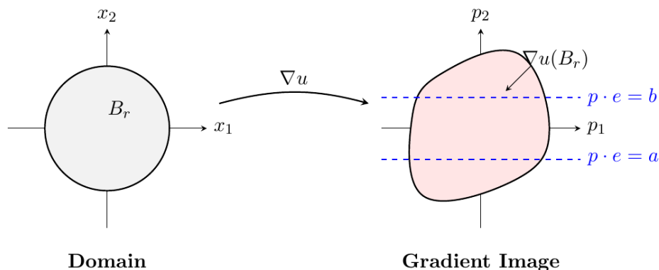
Figure 6: Chopping the gradient image with parallel strips in many directions forces \nabla u(B_r) to lie entirely on one side of each st
