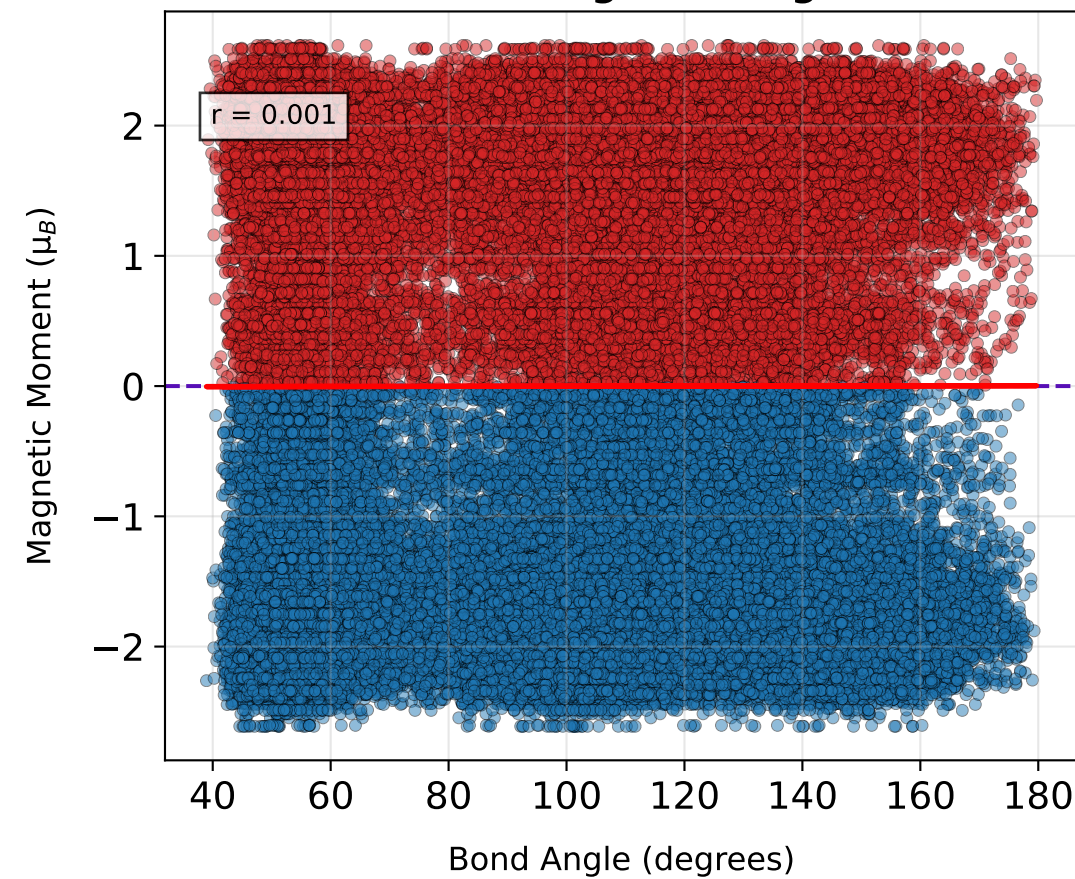
Fe-Fe-Ge: Angle vs Magmom
