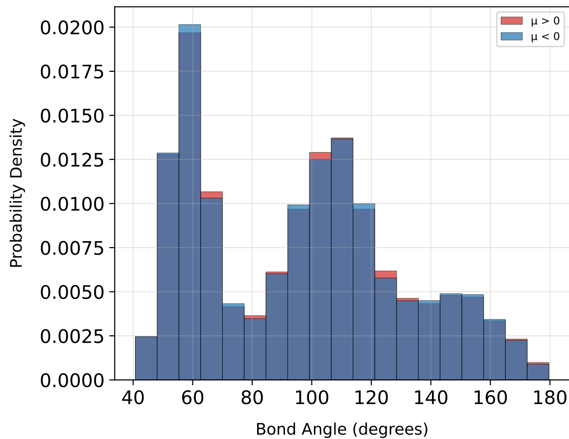
Fe-Fe-Fe: Angle vs Magmom
