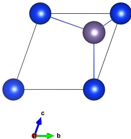
(e) SiGe (cubic)
