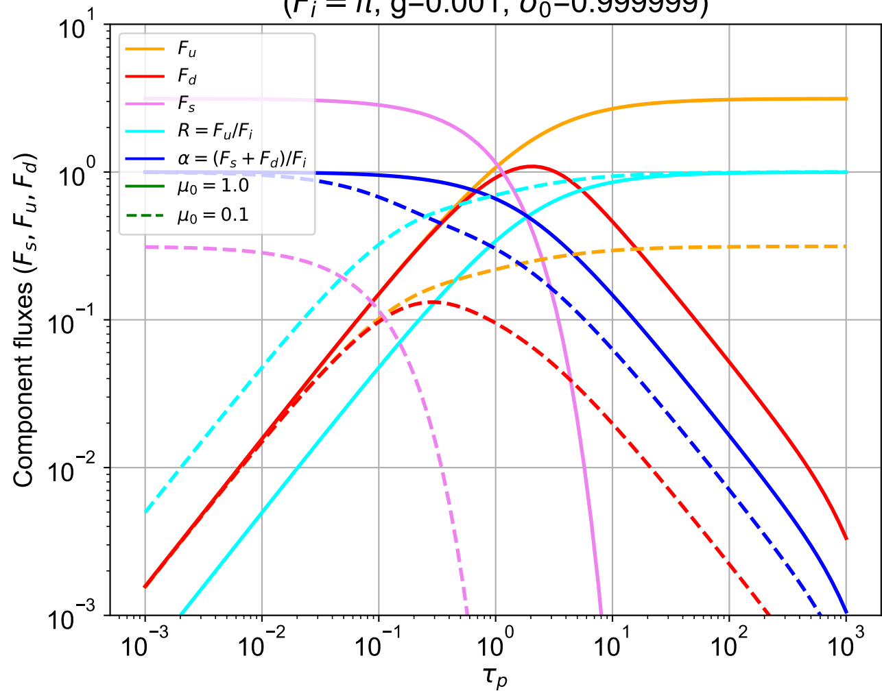
Different fluxes vs acoustic thickness ( F_i = \pi , g=0.001 , \sigma_0=0.999999 )
