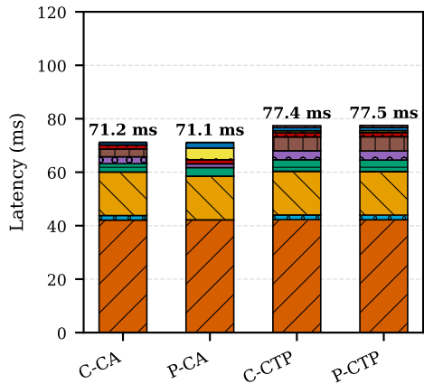
(a) Low Security P-256 & ML-44
