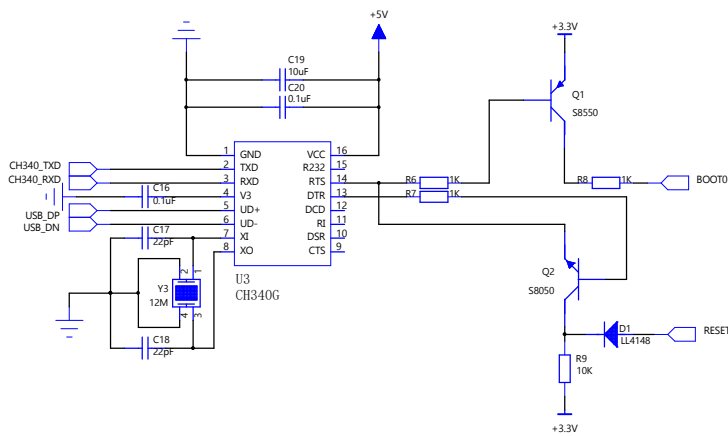
USB TO TTL
