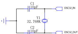
RTC时钟
