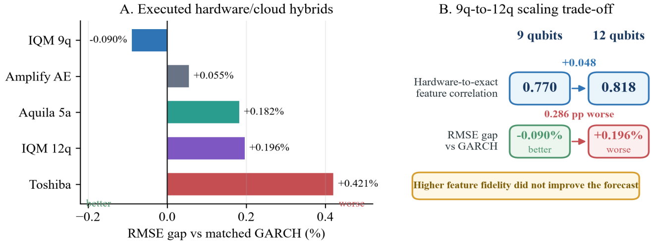
Figure 3. Negative RMSE gap is better. Panel B shows that higher 12-qubit feature fidelity does not improve the forecast.
