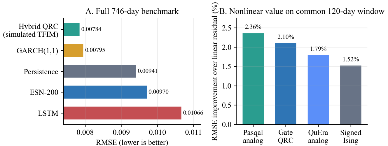
Figure 2. Left: the simulated TFIM hybrid is the advantage candidate. Right: every hardware-ready reservoir improves on the same linear residual ablation, although none beats GARCH on the common 120-day window.
