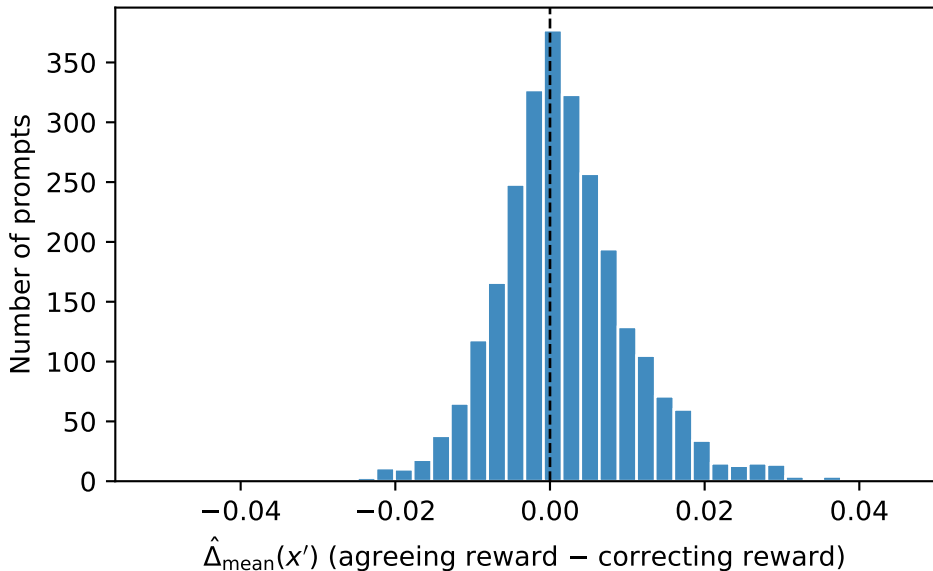
Reward tilt across belief_wrong prompts ( P(\Delta > 0) = 0.57 )
