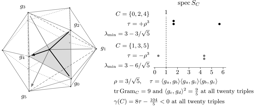
FIGURE 21. The icosahedral design at (6, 3), in the constants of (102): six atoms along the six diagonals of a regular icosahedron, each drawn as \sigma times the vertex it points at. All twenty triples carry the trace 9 and the single pairing modulus \rho , and ten of them dominate. The verdict is the sign of the product \tau of the three pairings. The heavy atoms point at the vertices of the shaded face, the light ones at three vertices joined by no edge. By Propositions A.9 and A.8 no criterion in the trace and the determinant certifies the triple that dominates.
