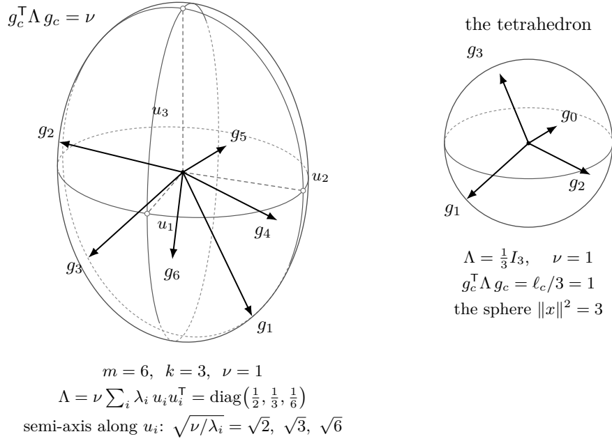
FIGURE 19. The quadric law (84). A stationarity datum confines every vector of its design to one central quadric of the multiplier, an ellipsoid whenever \Lambda is nonsingular. Drawn at (6, 3): the six vectors of a design, all on the ellipsoid of \Lambda = \text{diag}(\frac{1}{2}, \frac{1}{3}, \frac{1}{6}) at \nu = 1 , with its three principal sections and its silhouette. By (86) the surface is assembled from the tight directions, the semi-axis along u_i having length \sqrt{\nu/\lambda_i} : it is longest where the multiplier mass is least. Inset: at the tetrahedron of Example 8.9 the multiplier is \frac{1}{3} I_3 and the quadric is the sphere \|x\|^2 = 3 .
