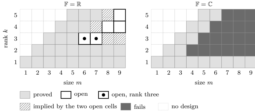
FIGURE 1. The decision board. Rows are the rank k , columns the size m ; cells with m < k carry no design. Over \mathbb{R} the two open cells at rank three are (6, 3) and (7, 3) ; the hatched region reduces to them by Theorem 5.15. Over \mathbb{C} the answer is m \leq k + 1 for every k \geq 2 .
