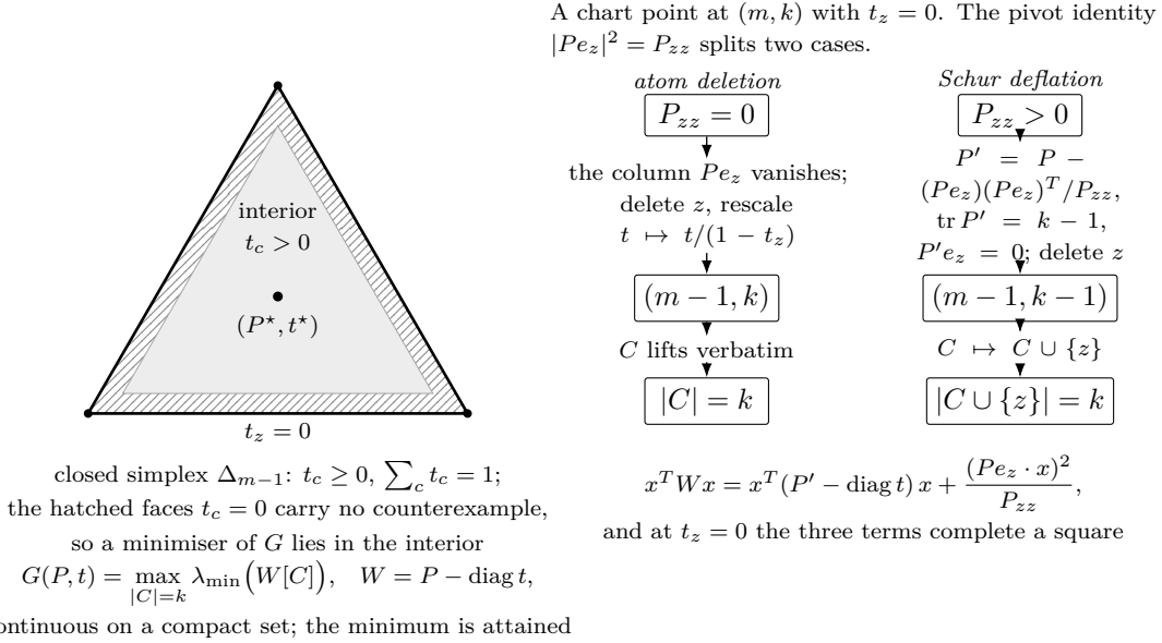
FIGURE 7. The compactification and the boundary dichotomy. Left: the objective G of (60) is continuous on a compact space, so it attains its minimum; Theorem 7.14 empties the faces t_z = 0 of counterexamples, which places the minimum in the interior. Right: the two mechanisms, separated by the pivot identity (63). At P_{zz} = 0 the atom is deleted and the weights rescaled; at P_{zz} > 0 the point is deflated by (65) and the selected subset regains z , the deficit in (67) being absent exactly because t_z = 0 .
