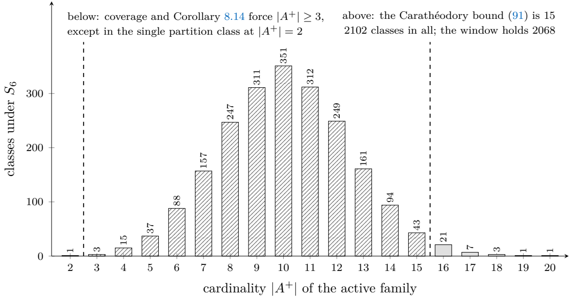
FIGURE 9. The census of Proposition 8.20 at (6, 3) . The active family covers \{1, \dots, 6\} , so it has at least two members, and the one class of cardinality two is the partition that Corollary 8.14 leaves undecided; (91) removes the classes above fifteen.
