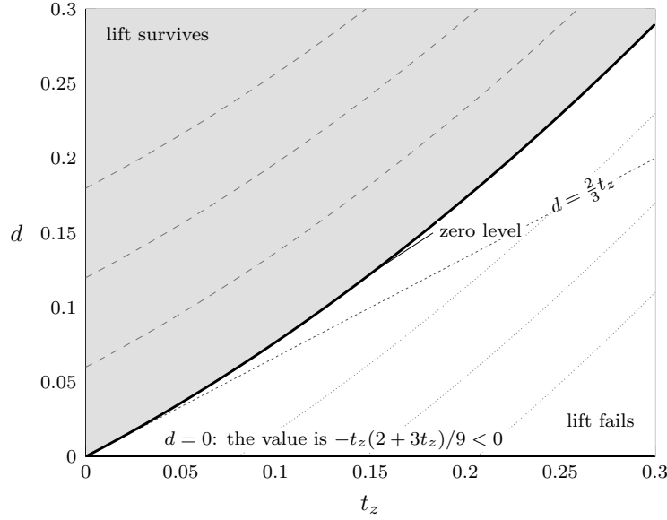
On the chart of Example 7.20 identity (68) reads \det W[\{c, z\}] = (3d - 2t_z - 3t_z^2)/9 , with zero level d = \frac{2}{3}t_z + t_z^2 . Dotted: the levels -\frac{1}{50}, -\frac{1}{75}, -\frac{1}{150} . Dashed: their positives.
