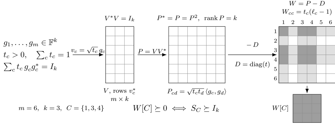
FIGURE 3. The chart, at m = 6 , k = 3 and C = \{1, 3, 4\} . The design data pass through the isometry V of (12) to the projection P = VV^* of (13) and the gap W = P - D of (14). Selecting C is taking a principal block, and Lemma 3.6 identifies its semidefiniteness with domination.
