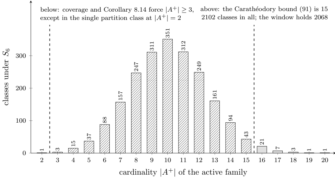
FIGURE 9. The census of Proposition 8.20 at (6, 3) . The active family covers \{1, \dots, 6\} , so it has at least two members; Corollary 8.14 removes the single class of cardinality two except in its partition branch, and (91) removes the classes above fifteen.
