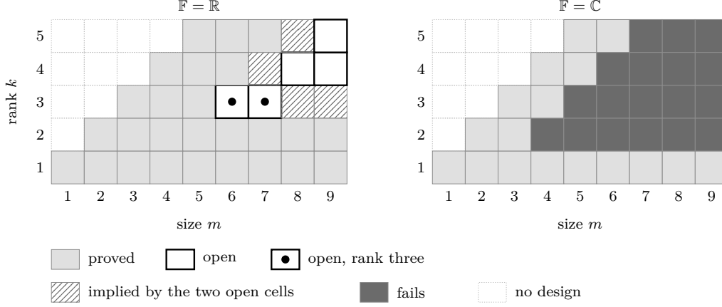
FIGURE 1. The decision board. Rows are the rank k , columns the size m ; cells with m < k carry no design. Over \mathbb{R} the two open cells at rank three are (6,3) and (7,3) ; the hatched region reduces to them by Theorem 5.15. Over \mathbb{C} the answer is m \leq k + 1 for every k \geq 2 .
