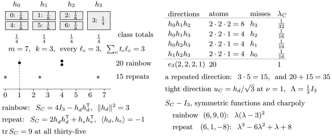
FIGURE 26. The split tetrahedron at (7, 3) of Example 6.7, and all thirty-five of its triples on one eigenvalue axis. Top left: the seven atoms by direction class, three classes of two and one of one, each carrying total weight \frac{1}{4} ; the count on the right runs over the resulting multiplicities (2, 2, 2, 1) . Bottom left: both spectra on one axis with the threshold dashed, the twenty triples that meet three directions on the upper row and the fifteen that repeat one below, singular on the line orthogonal to the two directions they carry. Right: the multipliers of the stationarity datum of Example 8.18, positive and summing to one; they are also the volume-sampling probabilities (55) of the same triples, \pi_C = (\prod_{c \in C} t_c) \cdot 16 . The lower spectrum is computed here, and of the three symmetric functions behind it the development carries the first and the last.
