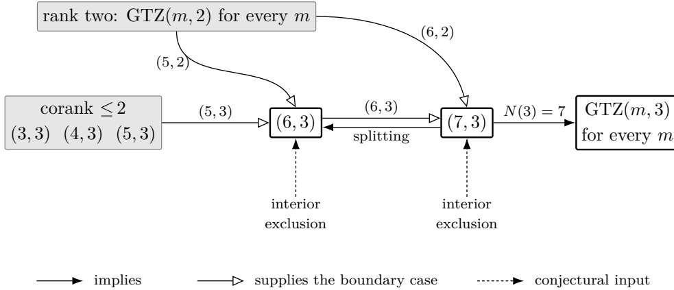
FIGURE 25. Rank three. The box on the left is Corollary 5.12; the filled arrows are Proposition 5.17 and Theorem 5.15; the open arrows are the boundary analysis of §7, which at a cell consumes the two cells one size below. Dashed arrows carry the two unproved inputs of §8.
