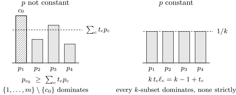
FIGURE 14. Theorem 3.21 at (4, 3) . The ratios p_c of (18) have co-weighted mean 1/k by (19). Left: the largest p_{c_0} is at least the t -weighted mean \sum_c t_c p_c , so by (20) its complement dominates. Right: when p is constant every p_c equals 1/k , the tie law (21) holds, every k -subset dominates and none dominates strictly.
