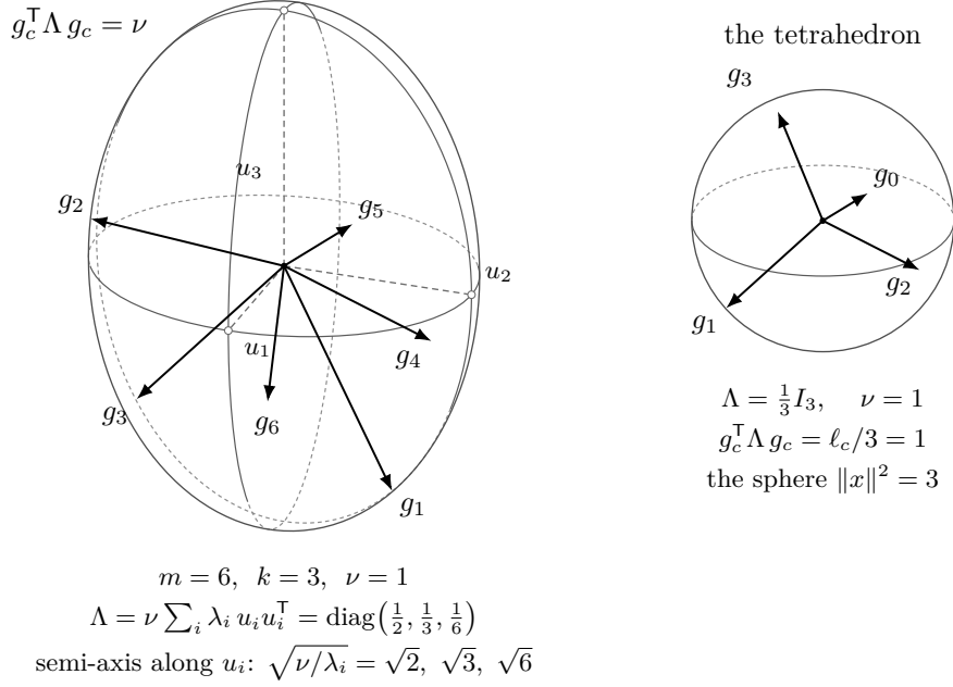
FIGURE 38. The quadric law (84). A stationarity datum confines every vector of its design to one central quadric of the multiplier, an ellipsoid whenever \Lambda is nonsingular. Drawn at (6, 3) : the six vectors of a design, all on the ellipsoid of \Lambda = \text{diag}(\frac{1}{2}, \frac{1}{3}, \frac{1}{6}) at \nu = 1 , with its three principal sections and its silhouette. By (86) the surface is assembled from the tight directions, the semi-axis along u_i having length \sqrt{\nu/\lambda_i} : it is longest where the multiplier mass is least. Inset: at the tetrahedron of Example 8.4 the multiplier is \frac{1}{3} I_3 and the quadric is the sphere \|x\|^2 = 3 .
