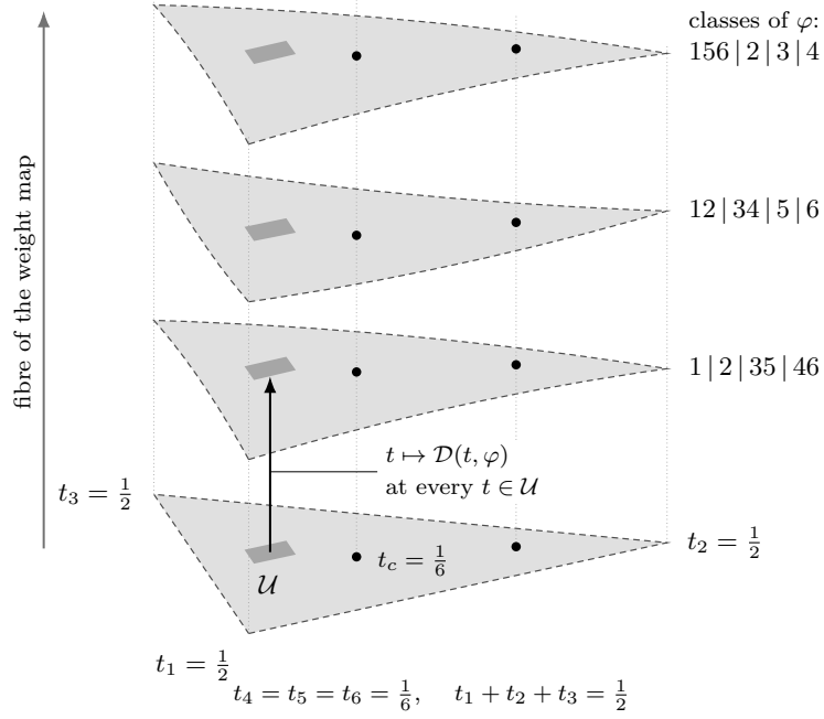
FIGURE 27. The equality locus as a section, at (6, 3) . Floor: the slice t_4 = t_5 = t_6 = \frac{1}{6} of the open weight simplex, its excluded boundary dashed and the uniform point marked. Vertical: the fibre of the weight map, drawn as a single dimension. Each sheet is a section t \mapsto \mathcal{D}(t, \varphi) of Proposition 6.5 restricted to that slice; the section is defined at every weight vector and its image has dimension m - 1 = 5 , the dimension of the weights. One sheet occurs for each partition of \{1, \dots, 6\} into four classes, 65 in all, of which three are drawn. However small, the shaded \mathcal{U} meets every one of them, so no restriction of the weights isolates a region on which the slack has a positive infimum; four of the nine strategies of Appendix A fail on that account.
