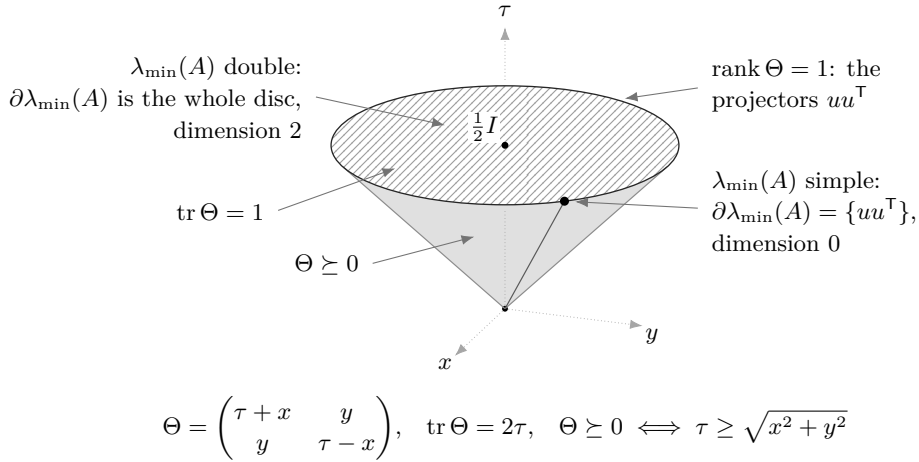
FIGURE 36. The spectraplex (75) at k = 2 . Trace one cuts the cone in a horizontal disc of radius \frac{1}{2} , whose boundary circle meets each extreme ray once and consists of the rank-one projectors. Since \lambda_{\min} is concave, (75) is a superdifferential; it is the face of that disc spanned by the unit eigenvectors at \lambda_{\min}(A) . The face at an eigenspace of dimension r has dimension \frac{1}{2}r(r+1) - 1 , so none has dimension one, and the multiplier attached to an active subset in Theorem 8.5 is a positive semidefinite matrix of trace one on the eigenspace rather than a scalar. Neither the spectraplex nor the passage of §8.3 from a local minimum to (73)–(74) is formal (§9.3).
