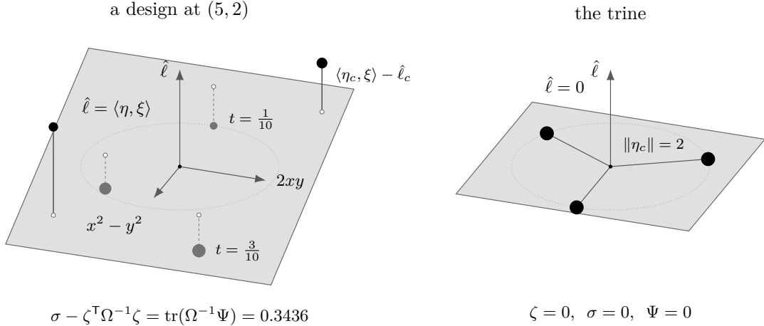
FIGURE 22. Lemma 5.9 as a fit. By (43) the slack \sigma - \zeta^\top \Omega^{-1} \zeta is the t -weighted squared residual of \hat{\ell} against the linear functional \langle \eta, \xi \rangle , \xi := \Omega^{-1} \zeta ; disc area is the weight, and an atom under the fitted plane carries a dashed segment. Left: an all-heavy design at (5, 2), where \det \Psi < 0 and \Psi is indefinite. Right: the trine of Example 5.4, where \hat{\ell} vanishes identically and the fit is exact.
