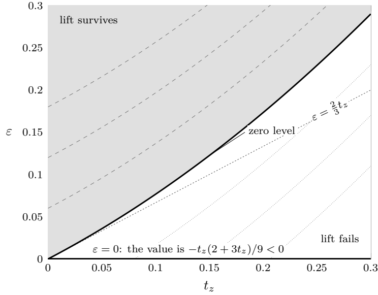
On the chart of Example 7.22 identity (68) reads \det W[\{c, z\}] = (3\varepsilon - 2t_z - 3t_z^2)/9 , with zero level \varepsilon = \frac{2}{3}t_z + t_z^2 . Dotted: the levels -\frac{1}{50}, -\frac{1}{25}, -\frac{3}{50} . Dashed: their positives.
