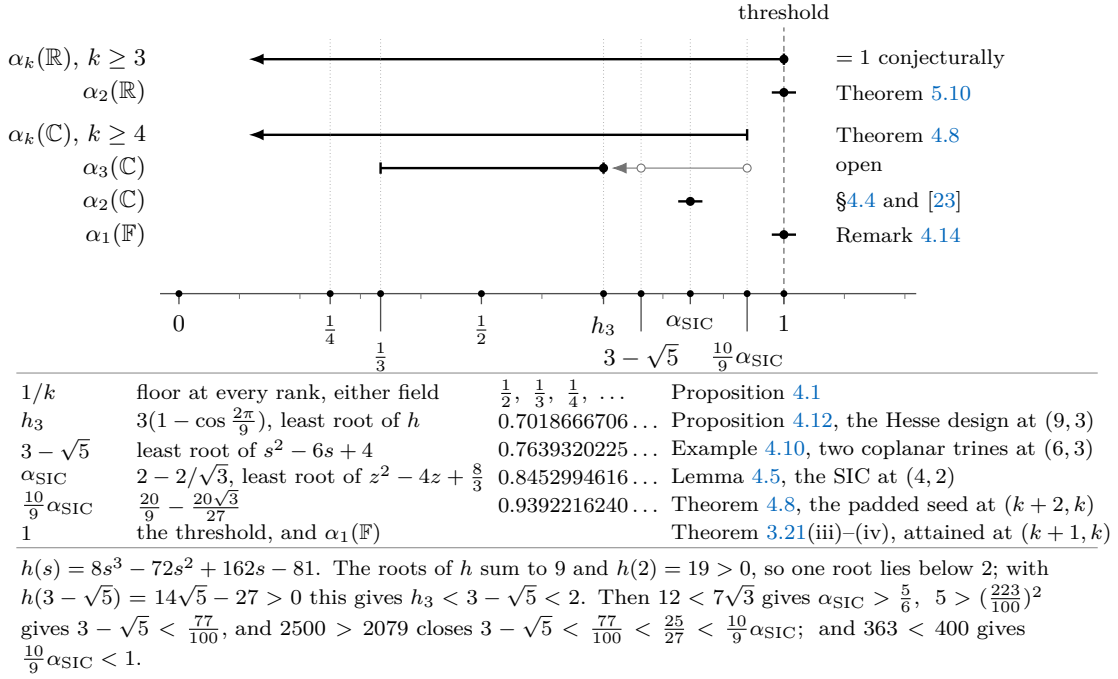
FIGURE 19. The six constants of §4 on one axis. Below the axis, the ledger giving each its exact form and, for three of them, a polynomial it is the least root of: the floor 1/k , the Hesse record h_3 , the trine value 3 - \sqrt{5} , the seed value \alpha_{\text{SIC}} , the padded bound \frac{10}{9}\alpha_{\text{SIC}} , and the threshold 1. Above it each rank carries the interval its two ends close, a filled dot marking an end attained by a design and an arrowhead an end running to 0 with 1/k . Rank two over \mathbb{C} is a point, while rank three spans [\frac{1}{3}, h_3] and stays open: the light arrow on that row is the record of Remark 4.14 moving down through \frac{10}{9}\alpha_{\text{SIC}} and 3 - \sqrt{5} without pinning anything. The lower end that pins \alpha_2(\mathbb{C}) is [23] at uniform weights carried to arbitrary weights in §4.4, and the top row's \alpha_k(\mathbb{R}) = 1 is the conjecture; what is proved on that row is the bracket [1/k, 1] together with a design whose value is exactly 1.
