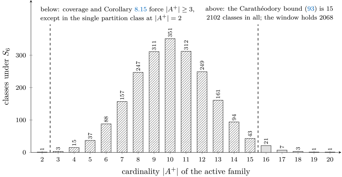
FIGURE 39. The census of Proposition 8.21 at (6, 3) . The active family covers \{1, \dots, 6\} , so it has at least two members, and the one class of cardinality two is the partition that Corollary 8.15 leaves undecided; (93) removes the classes above fifteen.
