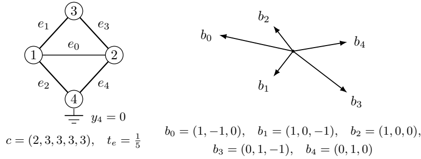
FIGURE 28. The diamond \mathcal{D}_\diamond . Left: the graph K_4 with the edge 34 deleted and the vertex 4 grounded, its edges carrying the conductances c = (2, 3, 3, 3, 3) and the uniform weights t_e = \frac{1}{5} ; line weight is proportional to conductance. Right: the five reduced incidence vectors of (49), pairwise non-proportional, whence the five atoms (51) are pairwise non-parallel.
