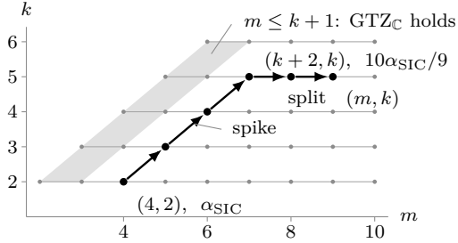
FIGURE 16. The two operations of §4.4, and the ladder they compose. Above: the matrix A of a design has c -th row g_c^H and satisfies A^H D A = I_k ; the spike borders it with one column and one row, the split repeats one row, and in each case the bordered Parseval product is the identity of the new rank. The spike divides the value bound by 1-w and the split leaves it alone, which is the whole cost accounting of Theorem 4.8. Below: the cells (m, k) for 2 \leq k \leq 6 , the shaded band m \leq k+1 where \text{GTZ}_{\mathbb{C}} holds by Proposition 4.2, and the staircase at (9, 5) : three spikes up the diagonal m = k+2 , then two splits along k = 5 . The tabulated w = 1 - (\frac{9}{10})^{1/e} gives (1-w)^e = \frac{9}{10} at every rank, so the bound after the spikes is \frac{10}{9}\alpha_{\text{SIC}} whatever k is, and since b < b/(1-w) for every b > 0 and every admissible w no member of the family attains b .
