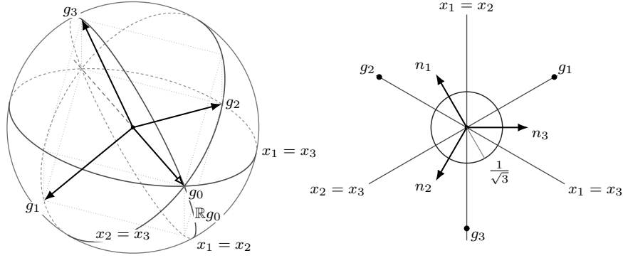
FIGURE 8. The certificate of Example 2.11 at the triple C = \{1, 2, 3\} . Each square (x_i - x_j)^2 vanishes on a plane spanned by g_0 and one selected atom, drawn left as its great circle on the circumsphere; the three planes meet in \mathbb{R}g_0 alone, the eigenline of S_C for the eigenvalue 1 of (10). Right: the same three planes seen along that line, six rays 60^\circ apart, with the unit normals n_c , signed to sum to zero, at 120^\circ and the level x^\top(S_C - I_3)x = 1 the circle of radius 1/\sqrt{3} of Figure 7. The grouping drawn is the one of Example 2.11; the development certifies the triple C = \{0, 1, 2\} instead, by the image of this certificate under \text{diag}(-1, -1, 1) , which permutes the atoms by (03)(12) .
