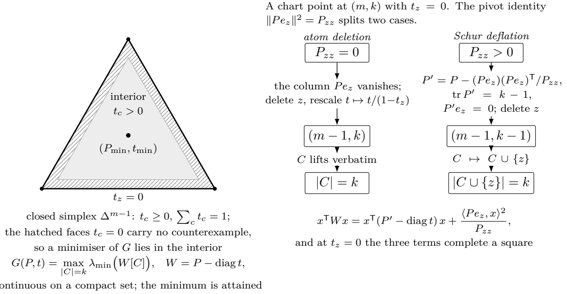
FIGURE 33. The compactification and the boundary dichotomy. Left: the objective G of (60) is continuous on a compact space, so it attains its minimum; Theorem 7.16 empties the faces t_z = 0 of counterexamples, which places a negative minimum in the interior. Right: the two mechanisms, separated by the pivot identity (63). At P_{zz} = 0 the atom is deleted and the weights rescaled; at P_{zz} > 0 the point is deflated by (65) and the selected subset regains z , the deficit in (67) being absent because t_z = 0 .
