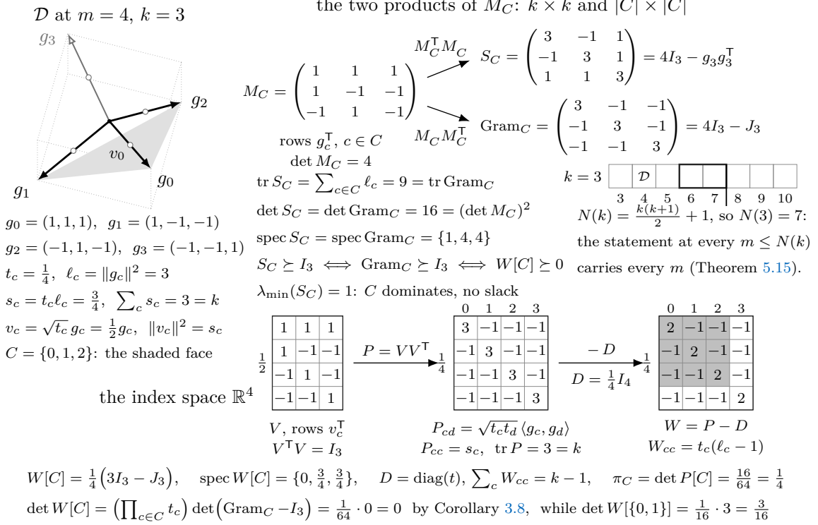
FIGURE 3. The reserved notation at the tetrahedron of Example 2.11. Left: the design, with C = \{0, 1, 2\} the shaded face, g_3 the omitted atom, and the chart atom v_c = \sqrt{t_c} g_c marked at half length on each arrow, where \|v_c\|^2 = s_c . Upper right: the two products of M_C of (11), different matrices of one trace, one determinant and one spectrum; the equivalence below them is Lemma 3.5 with Lemma 3.6, and holds at the one selection size |C| = k at which M_C is square. Bottom: the chart of (13), with the block W[C] shaded; its determinant is taken directly and again through Corollary 3.8, and the same reading at the pair \{0, 1\} returns \frac{3}{16} , so the 3 \times 3 minor vanishes and the 2 \times 2 one does not. The strip on the right places the design at m = 4 against the window N(3) = 7 and rings the two cells of Corollary 5.19. Every weight, leverage and leverage score is constant in c here, so the plate carries no variation across the atoms and no domination with positive slack.
