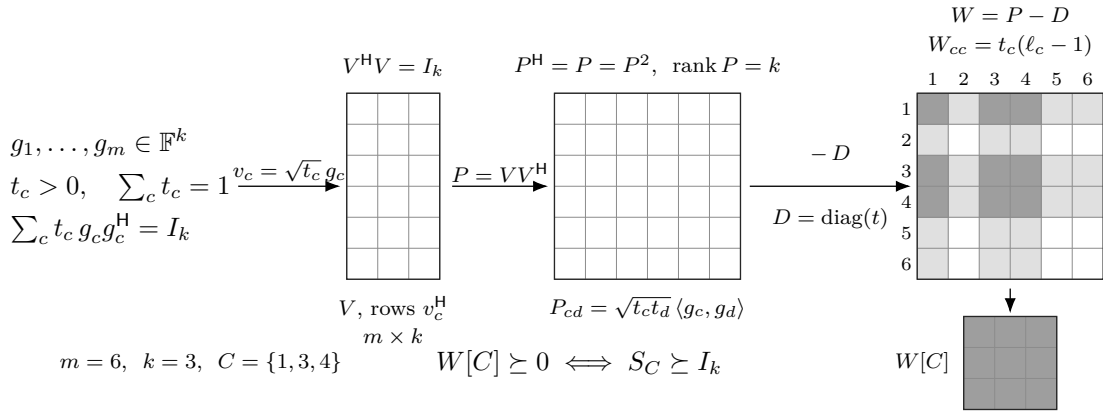
FIGURE 9. The chart, at m = 6 , k = 3 and C = \{1, 3, 4\} . The design data pass through the isometry V of (12) to the projection P = V V^H of (13) and the gap W = P - D of (14). Selecting C is taking a principal block, and Lemma 3.6 identifies its semidefiniteness with domination.
