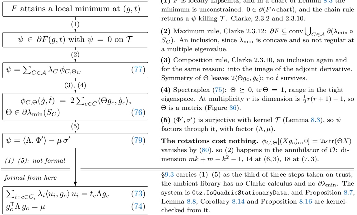
FIGURE 37. The assembly of (73)–(74). Left: the passage from a local minimum of F to the system in five steps, each arrow labelled by the rules that license it; the last carries no label, being the comparison of coefficients. Right: the rules. Two give inclusions rather than equalities, (2) and (3), for one reason: \lambda_{\min} is concave and so not Clarke regular where the least eigenvalue is multiple. Both inclusions run the direction a necessary condition needs. The infinitesimal rotations (72) impose nothing by (80), so the combination in (2) takes place in a space of dimension mk + m - k^2 - 1 , which is 14 at (6, 3) and 18 at (7, 3) and is where the bound (93) comes from. Nothing above the rule is formal: §9.3 carries the whole passage as one of three steps taken on trust, and the ambient library has no Clarke calculus and no \partial \lambda_{\min} .
