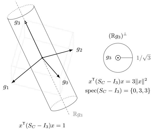
FIGURE 7. The gap S_C - I_3 at the triple C = \{0, 1, 2\} of Example 2.11. Left: the level set x^T(S_C - I_3)x = 1 , in the cube and the projection of Figure 6; the omitted atom g_3 carries an open head and spans the null line. Right: the same set seen along that line. Both nonzero eigenvalues of the gap equal 3 (§B.1), so the level set is a circular cylinder of radius 1/\sqrt{3} rather than a general elliptic one. Dominating with nothing to spare is a form singular along one line, and that line is spanned by the atom the triple omits (§6).
