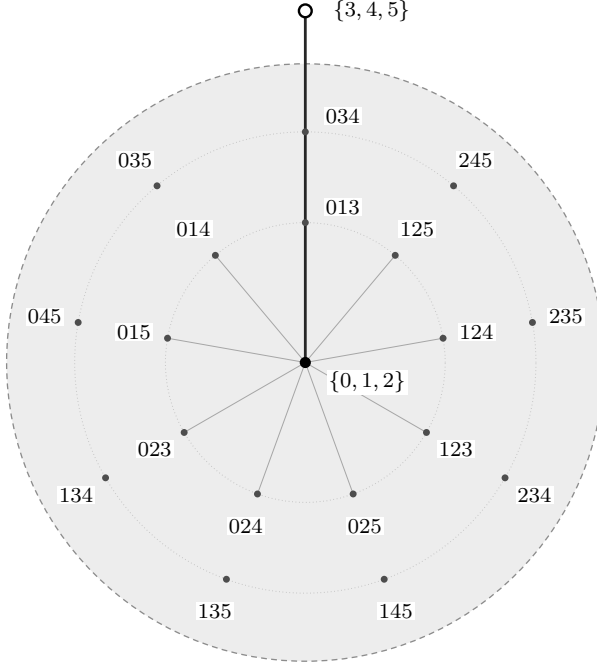
shells by exchange distance from \{0, 1, 2\} , of sizes 1 + 9 + 9 + 1 : the ball of radius two holds nineteen of the twenty triples and misses the one that dominates
