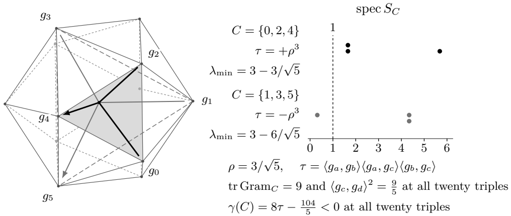
FIGURE 44. The icosahedral design at (6, 3) , in the constants of (102): six atoms along the six diagonals of a regular icosahedron, each drawn as \sigma times the vertex it points at. All twenty triples carry the trace 9 and the single pairing modulus \rho , and ten of them dominate. The verdict is the sign of the product \tau of the three pairings. The heavy atoms point at the vertices of the shaded face, the light ones at three vertices joined by no edge. By Propositions A.9 and A.8 no criterion in the trace and the determinant certifies the triple that dominates.
