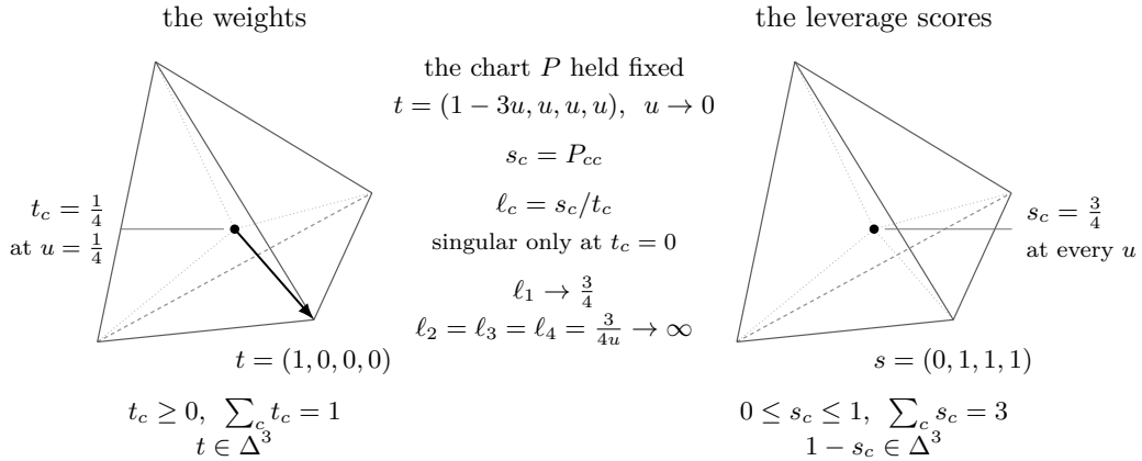
FIGURE 31. The two simplices at (4, 3) . Left: the weights, in \Delta^3 . Right: the leverage scores, confined by Lemmas 2.3 and 2.4 to \{s \in [0, 1]^4 : \sum_c s_c = 3\} , which at corank one is again \Delta^3 , in the coordinates 1 - s_c . The tetrahedron design of Example 2.11 is the barycentre of each. With its chart held fixed (Lemma 3.2) the weights run to a vertex while the leverage scores stand still, and the leverages \ell_c = s_c/t_c diverge; Example 7.1 is the same motion at (2, 1) . The leverage score is the coordinate that stays compact and the weight the one that reaches the boundary, so the compactification is taken in (P, t) rather than in the design data.
