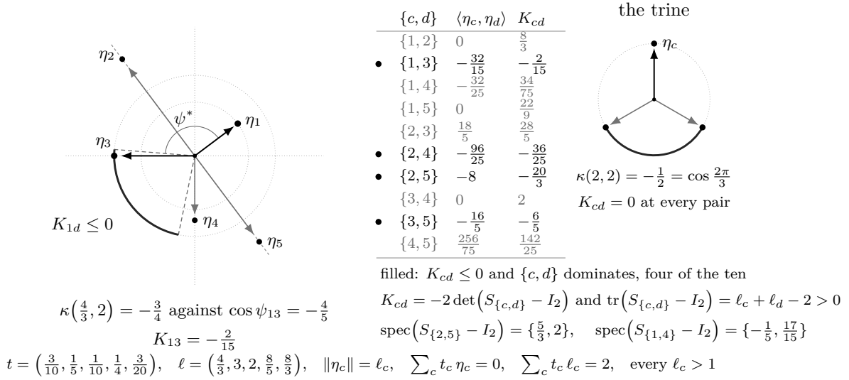
FIGURE 21. The pair obstruction (38) at (5, 2). Left: the squared vectors of an all-heavy design, at distance \ell_c from the origin. The two circles drawn are those of the pair \{1, 3\} , and the arc on the circle of radius \ell_3 = 2 carries the partners \eta_d with K_{1d} \leq 0 . Every point of that arc makes an angle of at least \psi^* with \eta_1 , where \cos \psi^* = \kappa(\ell_c, \ell_d) := [(\ell_c - 2)(\ell_d - 2) - 2]/(\ell_c \ell_d) ; both \kappa + 1 = 2(\ell_c - 1)(\ell_d - 1)/(\ell_c \ell_d) and 1 - \kappa = 2(\ell_c + \ell_d - 1)/(\ell_c \ell_d) are positive at a heavy pair, so the arc is proper and nonempty there and the two leverages by themselves decide no pair. Centre: the ten pairs, four of them dominating. Right: the trine of Example 5.4, where the cosine the design realizes and the threshold \kappa(2, 2) are both -\frac{1}{2} , so each pair sits at an endpoint of the arc and K_{cd} = 0 .
