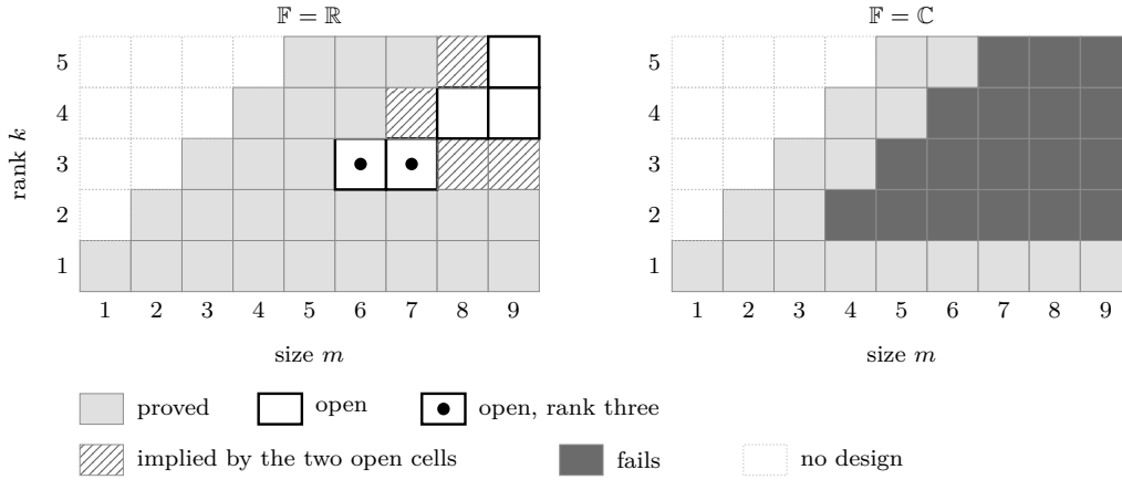
FIGURE 2. The decision board. Rows are the rank k , columns the size m ; cells with m < k carry no design. Over \mathbb{R} the two open cells at rank three are (6, 3) and (7, 3) ; the hatched region reduces to them by Theorem 5.15 and Corollary 3.16. Over \mathbb{C} the answer is m \leq k + 1 for every k \geq 2 .
