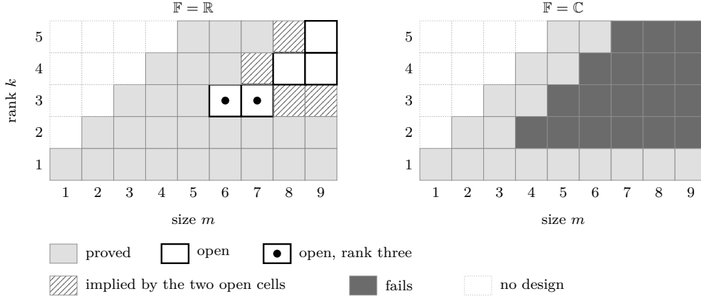
FIGURE 1. The decision board. Rows are the rank k , columns the size m ; cells with m < k carry no design. Over \mathbb{R} the two open cells at rank three are (6,3) and (7,3); the hatched region reduces to them by Theorem 5.15. Over \mathbb{C} the answer is m \leq k + 1 for every k \geq 2 .
