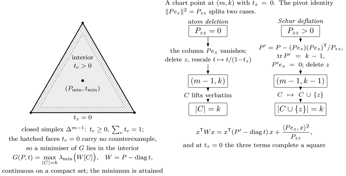
FIGURE 16. The compactification and the boundary dichotomy. Left: the objective G of (60) is continuous on a compact space, so it attains its minimum; Theorem 7.15 empties the faces t_z = 0 of counterexamples, which places a negative minimum in the interior. Right: the two mechanisms, separated by the pivot identity (63). At P_{zz} = 0 the atom is deleted and the weights rescaled; at P_{zz} > 0 the point is deflated by (65) and the selected subset regains z , the deficit in (67) being absent because t_z = 0 .
