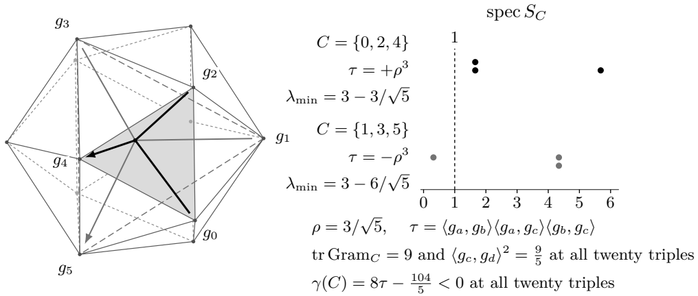
FIGURE 21. The icosahedral design at (6,3), in the constants of (102): six atoms along the six diagonals of a regular icosahedron, each drawn as \sigma times the vertex it points at. All twenty triples carry the trace 9 and the single pairing modulus \rho , and ten of them dominate. The verdict is the sign of the product \tau of the three pairings. The heavy atoms point at the vertices of the shaded face, the light ones at three vertices joined by no edge. By Propositions A.9 and A.8 no criterion in the trace and the determinant certifies the triple that dominates.
