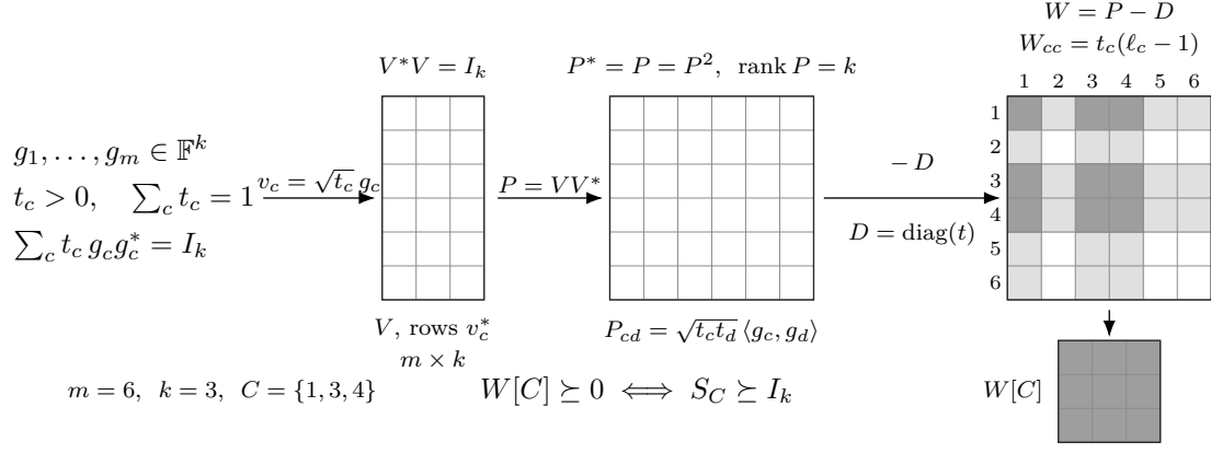
FIGURE 3. The chart, at m = 6, k = 3 and C = \{1, 3, 4\} . The design data pass through the isometry V of (12) to the projection P = VV^* of (13) and the gap W = P - D of (14). Selecting C is taking a principal block, and Lemma 3.6 identifies its semidefiniteness with domination.
