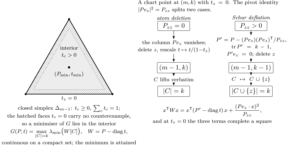
FIGURE 7. The compactification and the boundary dichotomy. Left: the objective G of (60) is continuous on a compact space, so it attains its minimum; Theorem 7.14 empties the faces t_z = 0 of counterexamples, which places the minimum in the interior. Right: the two mechanisms, separated by the pivot identity (63). At P_{zz} = 0 the atom is deleted and the weights rescaled; at P_{zz} > 0 the point is deflated by (65) and the selected subset regains z , the deficit in (67) being absent exactly because t_z = 0 .
