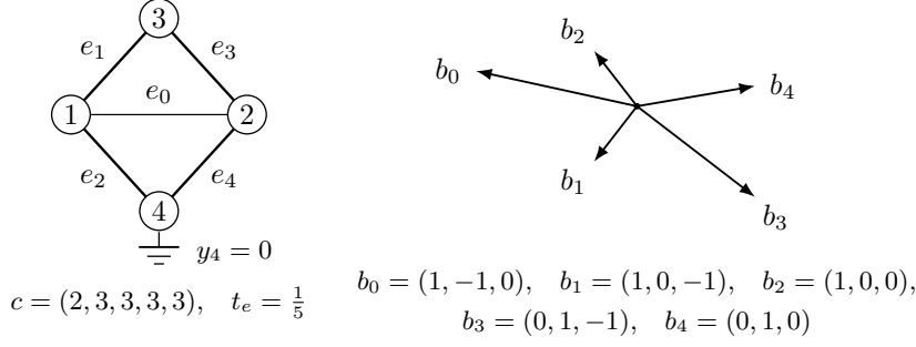
FIGURE 6. The diamond \mathcal{D}_\diamond . Left: the graph K_4 with the edge 34 deleted and the vertex 4 grounded, its edges carrying the conductances c = (2, 3, 3, 3, 3) and the uniform weights t_e = \frac{1}{5} ; line weight is proportional to conductance. Right: the five reduced incidence vectors of (49), pairwise non-proportional, whence the five atoms (51) are pairwise non-parallel.
