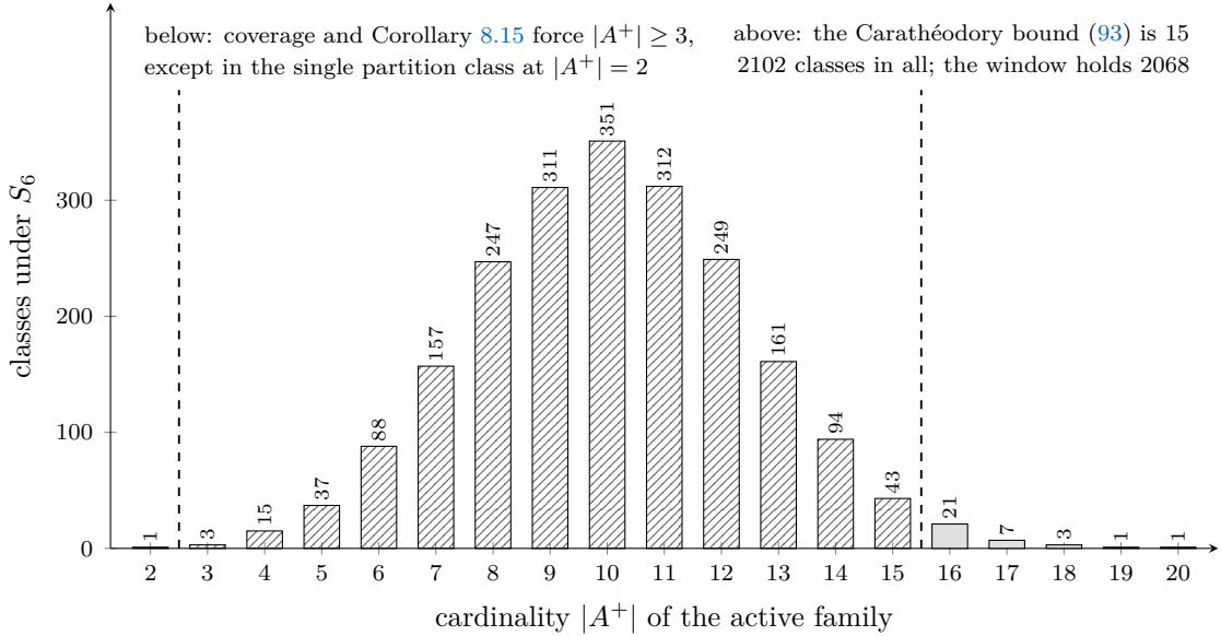
FIGURE 9. The census of Proposition 8.21 at (6, 3) . The active family covers \{1, \dots, 6\} , so it has at least two members, and the one class of cardinality two is the partition that Corollary 8.15 leaves undecided; (93) removes the classes above fifteen.
