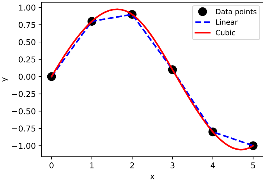
Interpolation Methods
