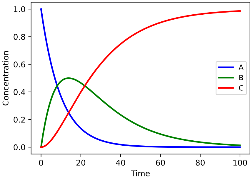
Consecutive Reactions: A \rightarrow B \rightarrow C
