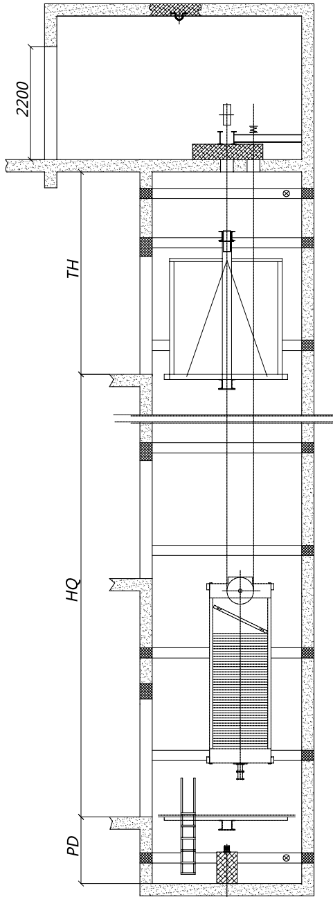
Hoistway vertical section
