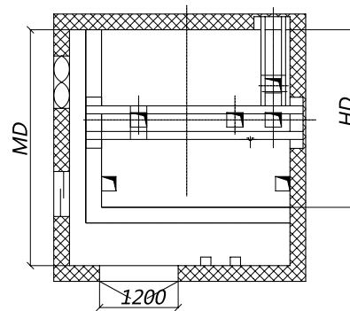
Machine room plan layout
