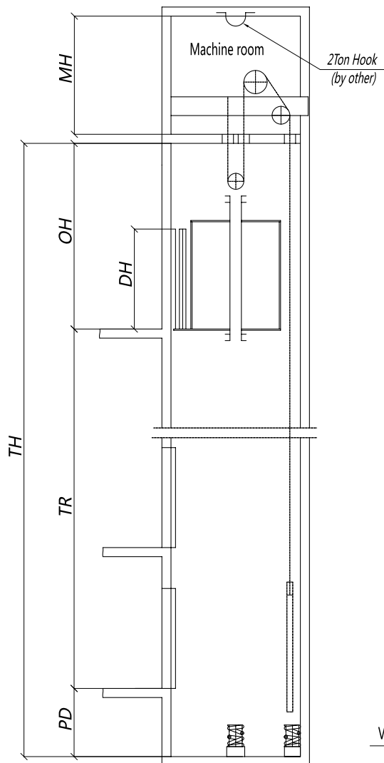
Hoistway vertical section
