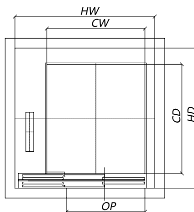
Hoistway plan layout (not breakthrough)
