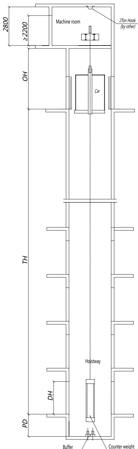
Hoistway vertical section
