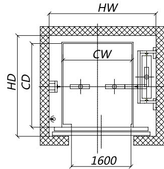
Hoistway plan layout (not breakthrough)
