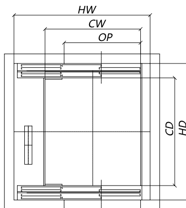
Hoistway plan layout (not breakthrough)
