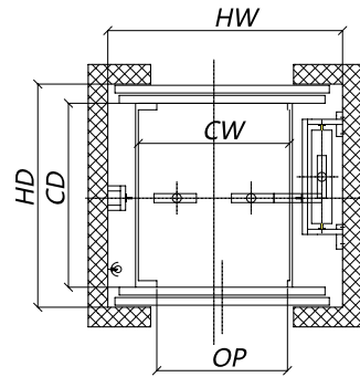
Hoistway plan layout (breakthrough)
