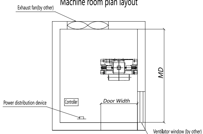
Machine room plan layout
