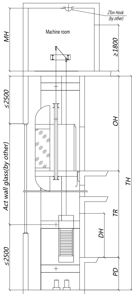
Hoistway vertical section
