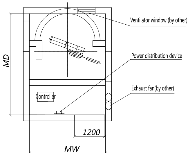
Machine room plan layout
